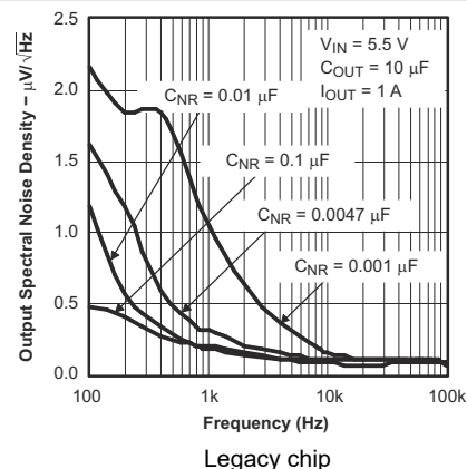
Figure 5-10. TPS79630-Q1 Output Spectral Noise Density vs Frequency
