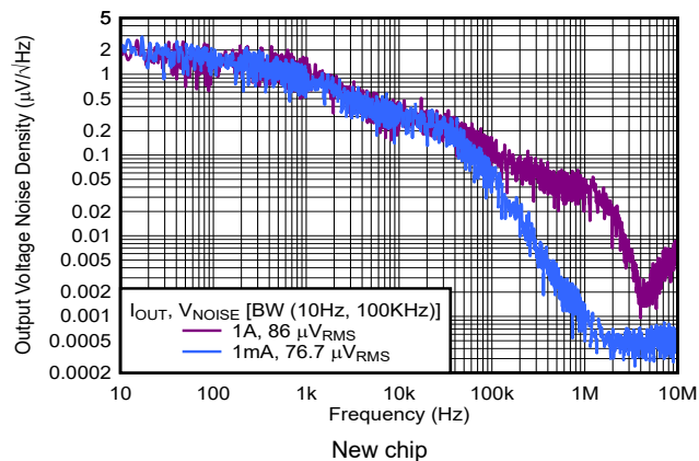
Figure 5-8. TPS79633-Q1 Output Spectral Noise Density vs Frequency
