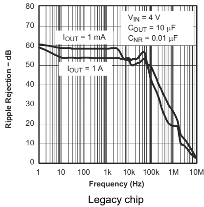
Figure 5-15. TPS79630-Q1 Ripple Rejection vs Frequency
