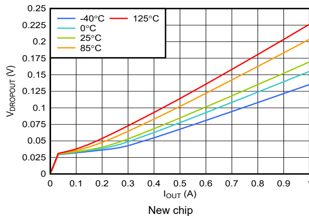
Figure 5-30. TPS79633-Q1 Dropout Voltage vs Output Current
