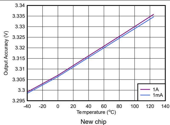
Figure 5-4. TPS79633-Q1 Output Voltage vs Junction Temperature
