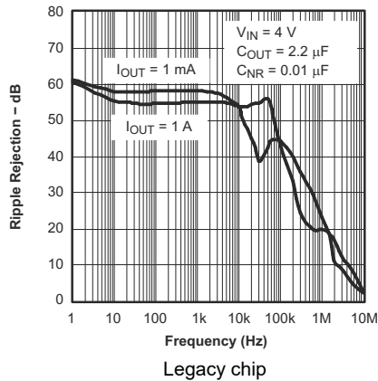
Figure 5-17. TPS79630-Q1 Ripple Rejection vs Frequency
