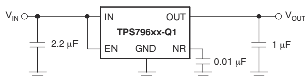
Figure 7-1. Typical Application Circuit (Legacy Chip)
