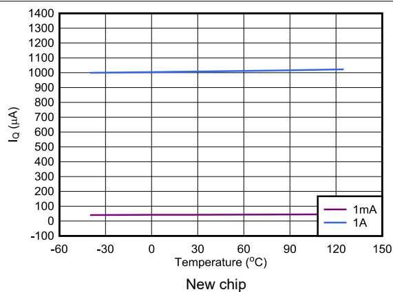
Figure 5-6. TPS79633-Q1 Ground Current vs Junction Temperature
