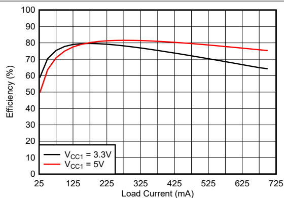
Figure 5-14. ISO774xTB-Q1 Efficiency vs. Load Current ISO774xTB-Q1 + Würth 750315371
