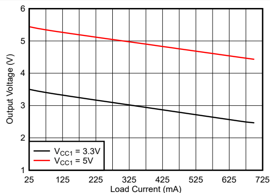
Figure 5-12. ISO774xTB-Q1 Output Voltage vs. Load Current ISO774xTB-Q1 + Würth 750315371
