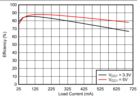
Figure 5-13. ISO774xTA-Q1 Efficiency vs. Load Current ISO774xTA-Q1 + Würth 750315240
