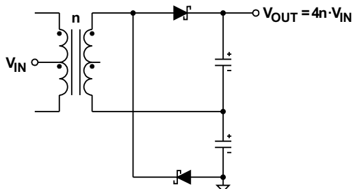
Figure 8-14. Half-Wave Rectifier Without Centered Ground and Center-Tapped Secondary Performs Voltage Doubling Twice, Hence Quadrupling V_{IN}
