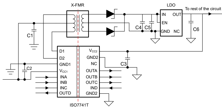
Simplified Schematic
