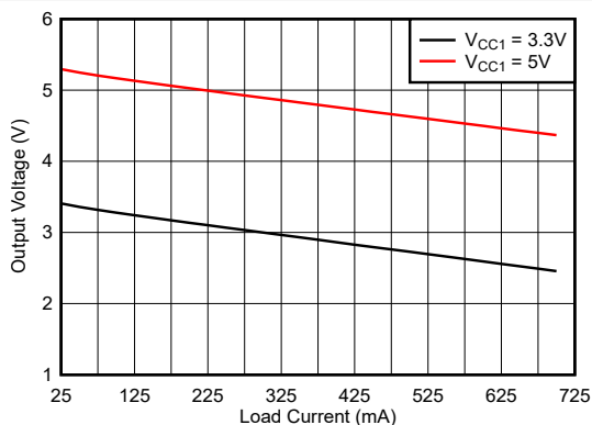
Figure 5-11. ISO774xTA-Q1 Output Voltage vs. Load Current ISO774xTA-Q1 + Würth 750315240
