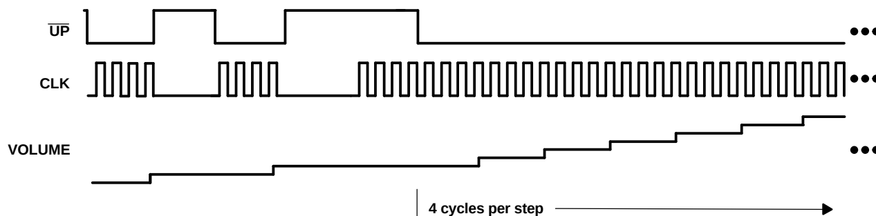
Figure 33. External Clock (4 Cycles Per Volume Change)
