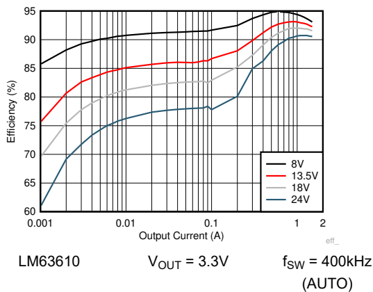
Figure 8-7. Efficiency
