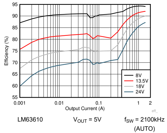
Figure 8-6. Efficiency
