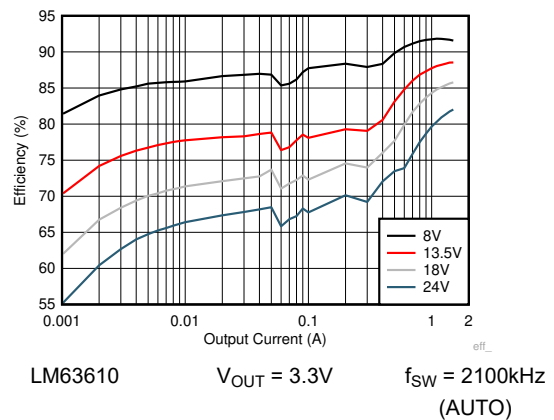
Figure 8-8. Efficiency
