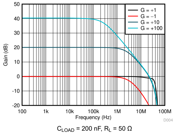
Figure 6-7. Closed-Loop Gain vs Frequency
