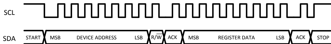
Figure 23. Example I²C Write Cycle
