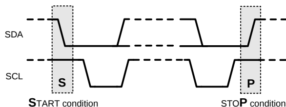
Figure 22. Start and Stop Diagram
