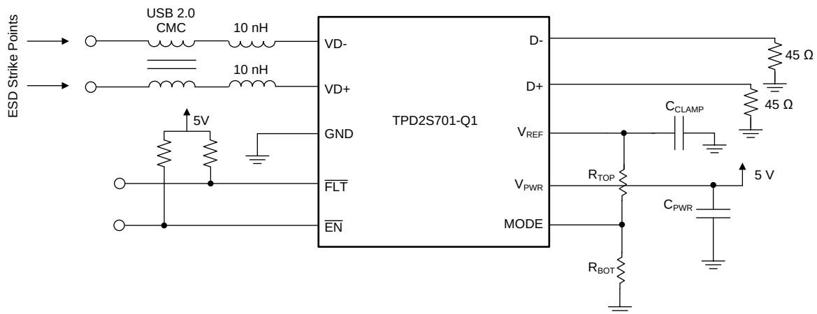
Figure 19. ESD Setup
