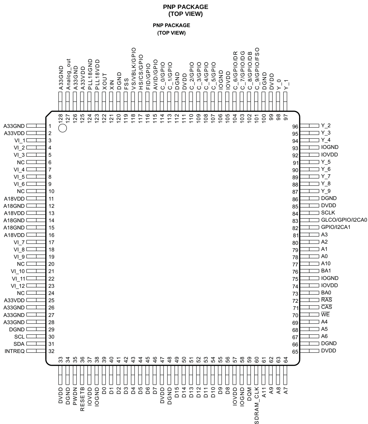
Figure 1-1. TVP5160 PNP-Package Terminal Diagram
