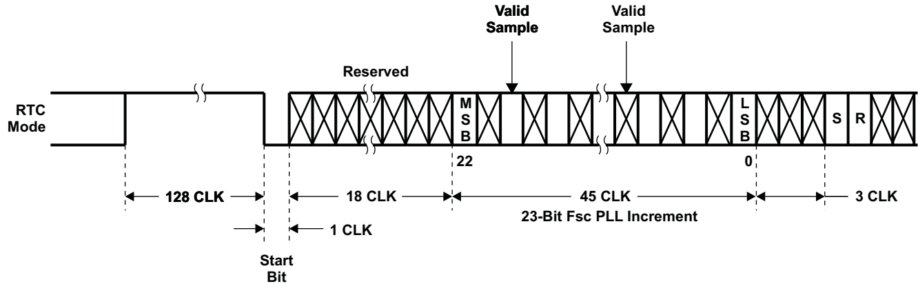
Figure 2-5. RTC Timing
