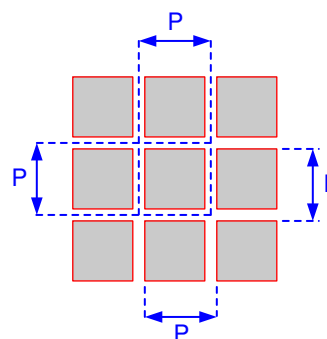
Figure 6-9. Micromirror Array Physical Characteristics
