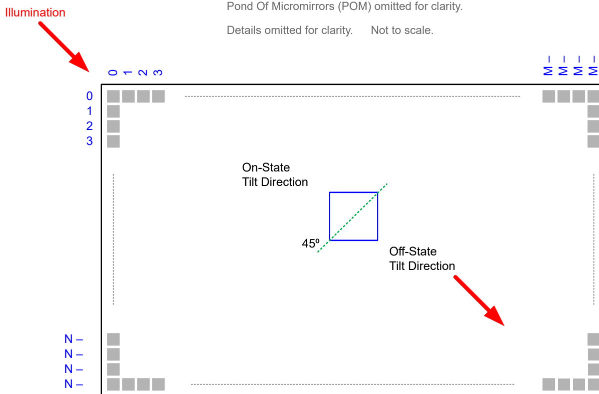
Figure 6-10. Micromirror Landed Orientation and Tilt
