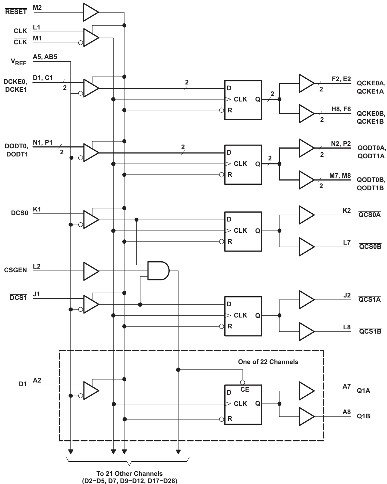
Logic Diagram for Register-A Configuration (Positive Logic); C = 0
