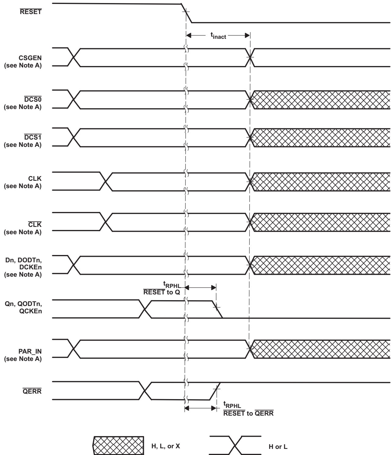
Timing Diagram for 74SSTUB32868 During Shut-Down ( \overline{\text{RESET}} Switches From H to L)
