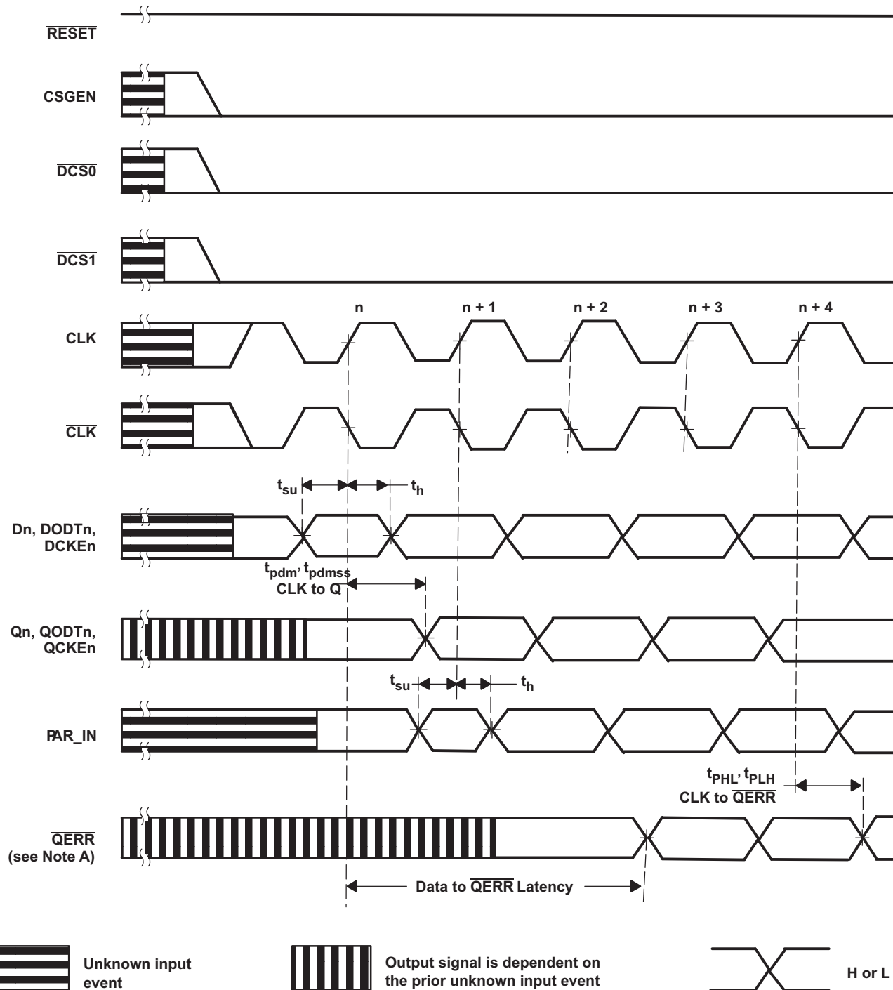
Timing Diagram for 74SSTUB32868 During Normal Operation ( \overline{\text{RESET}} = \text{H} )
