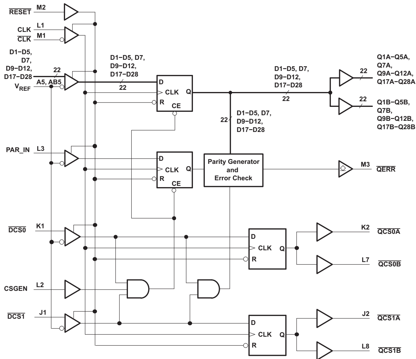
Parity Logic Diagram for Register-A Configuration (Positive Logic); C = 0
