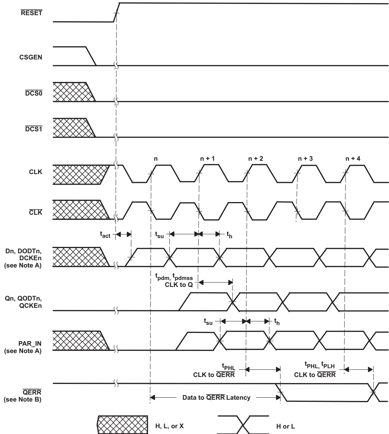
Timing Diagram for 74SSTUB32868 During Start-Up ( \overline{\text{RESET}} Switches From L to H)
