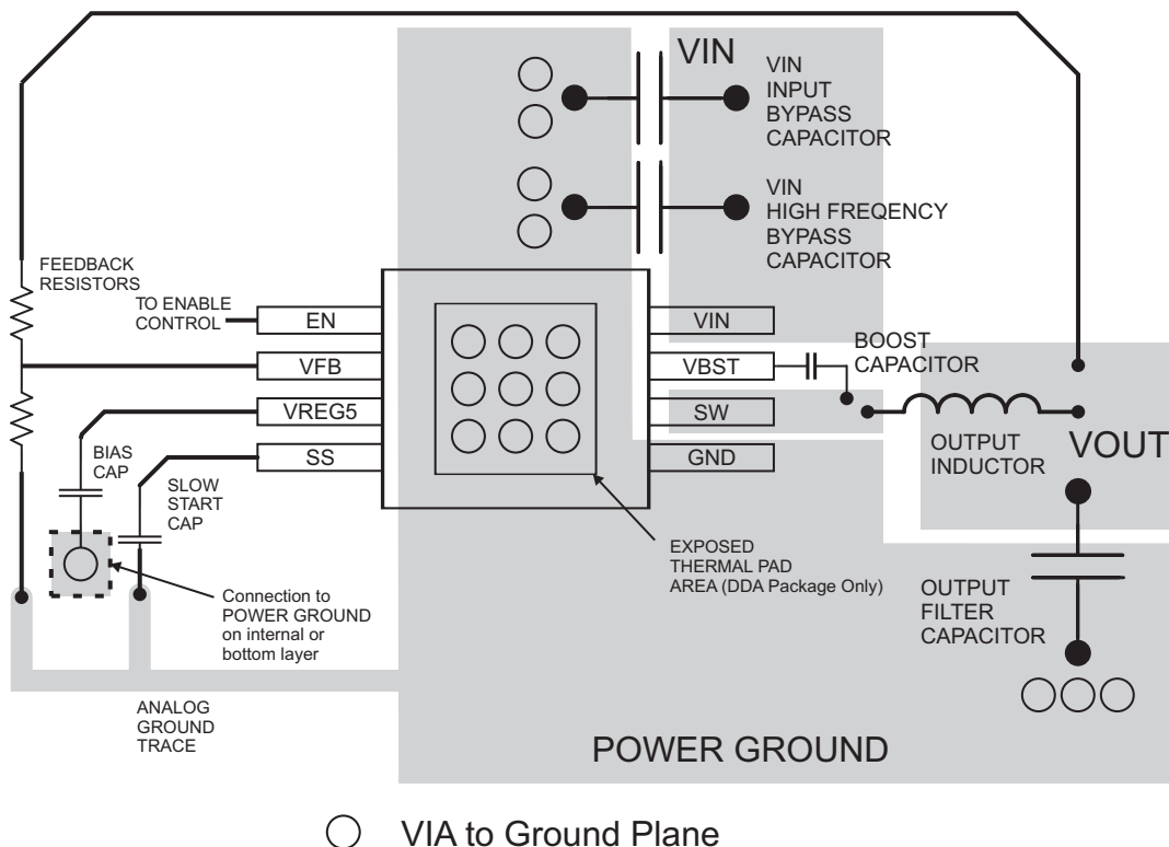
Figure 19. PCB Layout
