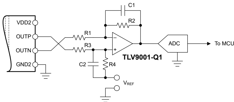
Figure 8-3. Connecting the AMC0x11D-Q1 Output to a Single-Ended Input ADC
