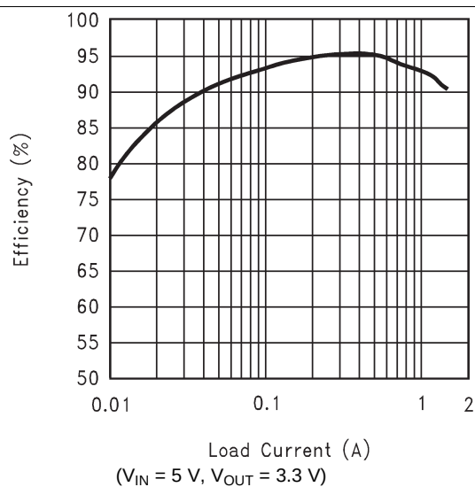
Figure 12. Efficiency vs Load Current
