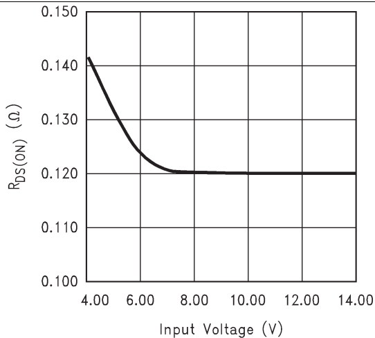
Figure 5. R_{DS(ON)} vs Input Voltage
