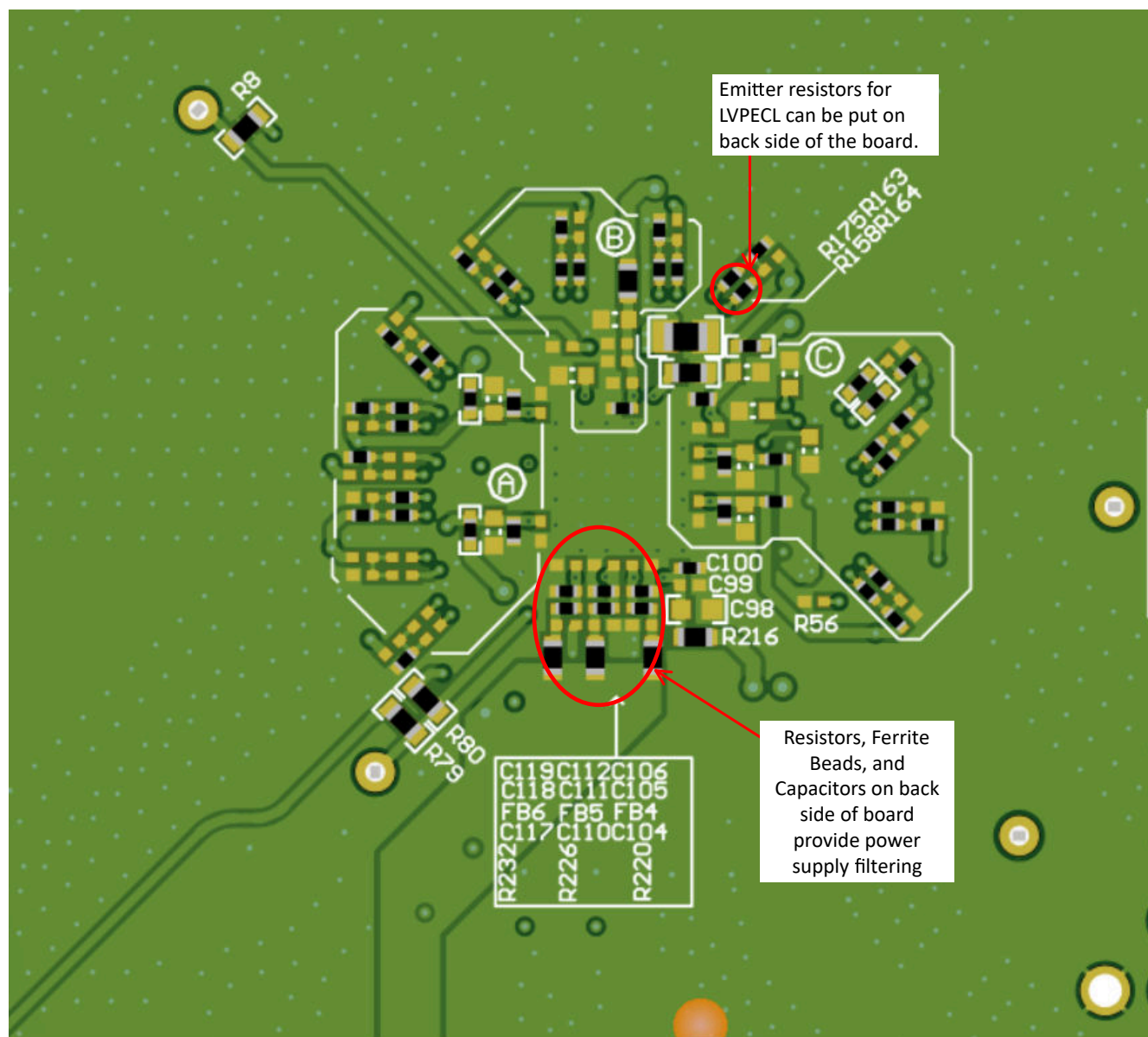
Figure 9-23. Bottom Layer
