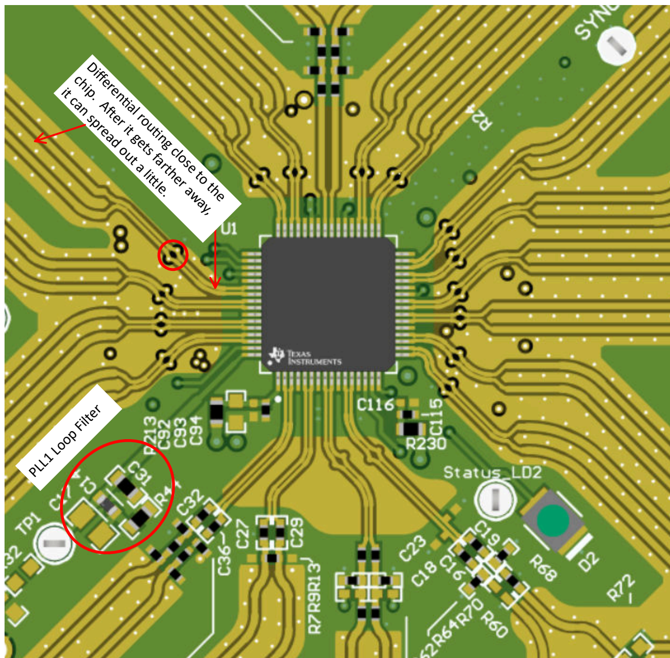
Figure 9-22. Top Layer
