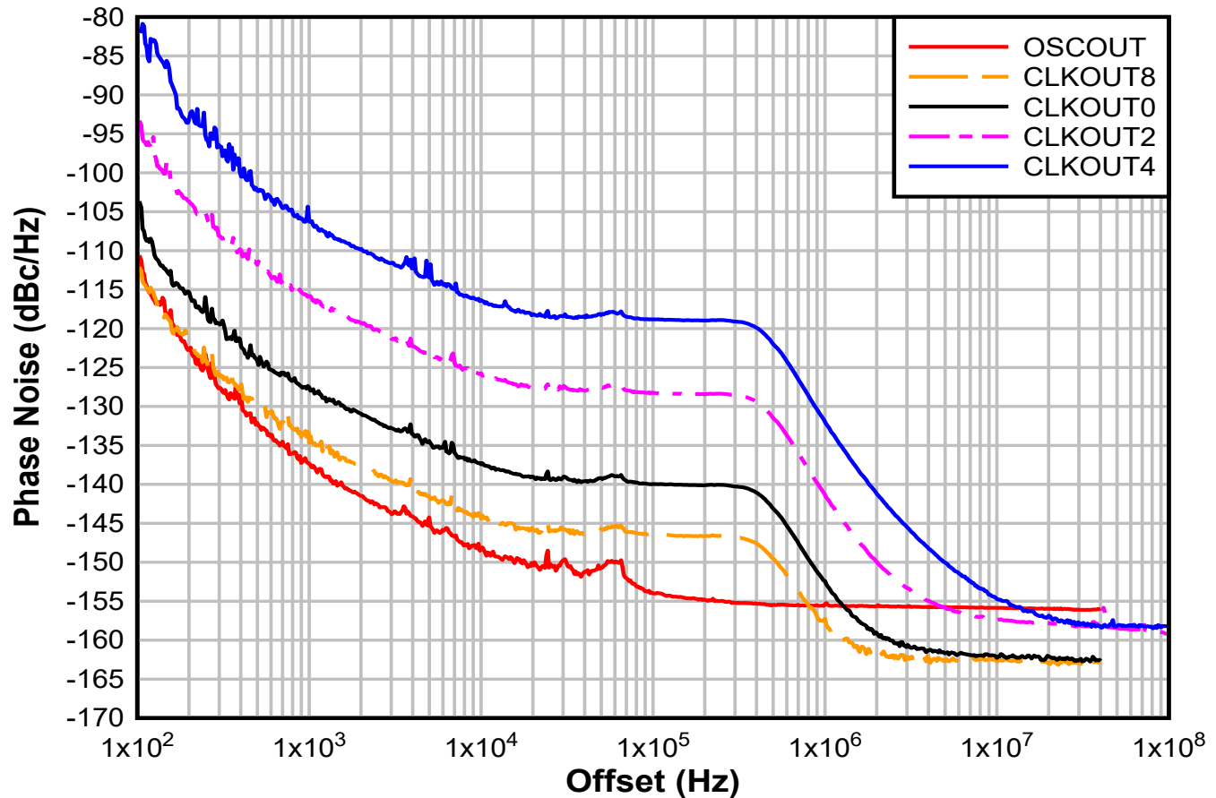
Figure 9-19. Offset vs Phase Noise
