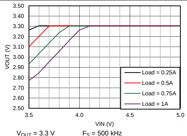
Figure 50. Dropout Curve
