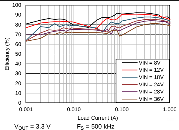
Figure 48. Efficiency
