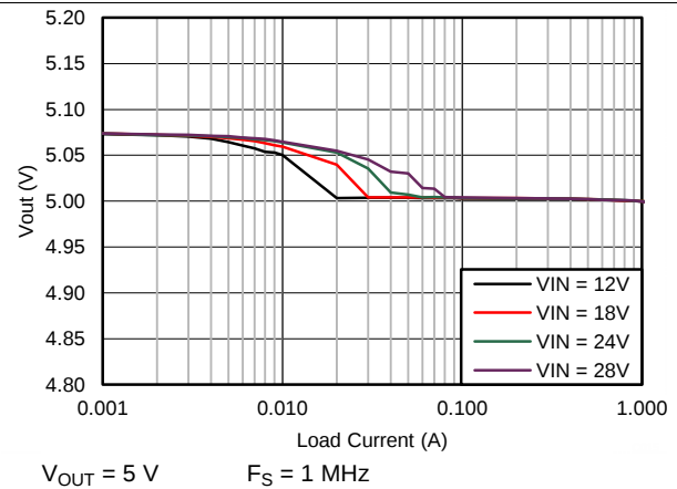
Figure 10. V_{OUT} Regulation
