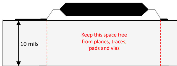
Figure 7-6. Layout Example - PCB Cross-Section
