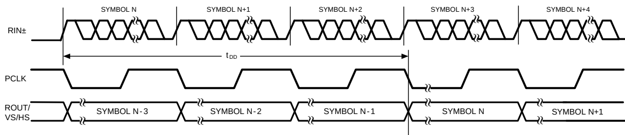
Figure 18. Deserializer Delay
