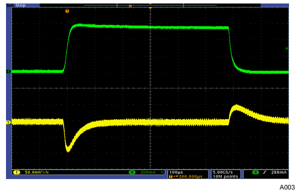
Figure 20. Load Transient Response, 10 mA to 550 mA
