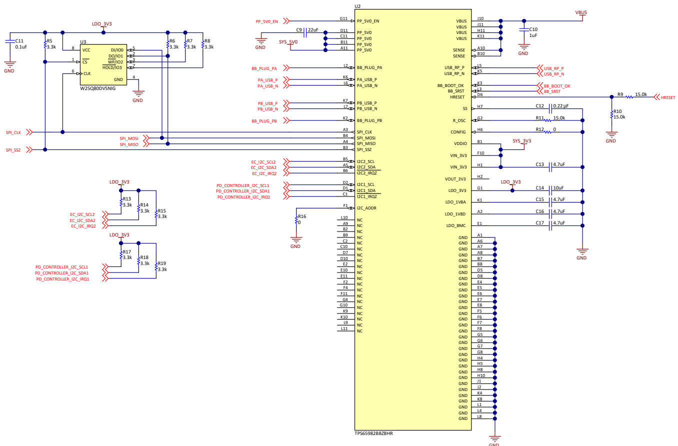
Figure 21. Example Schematic
