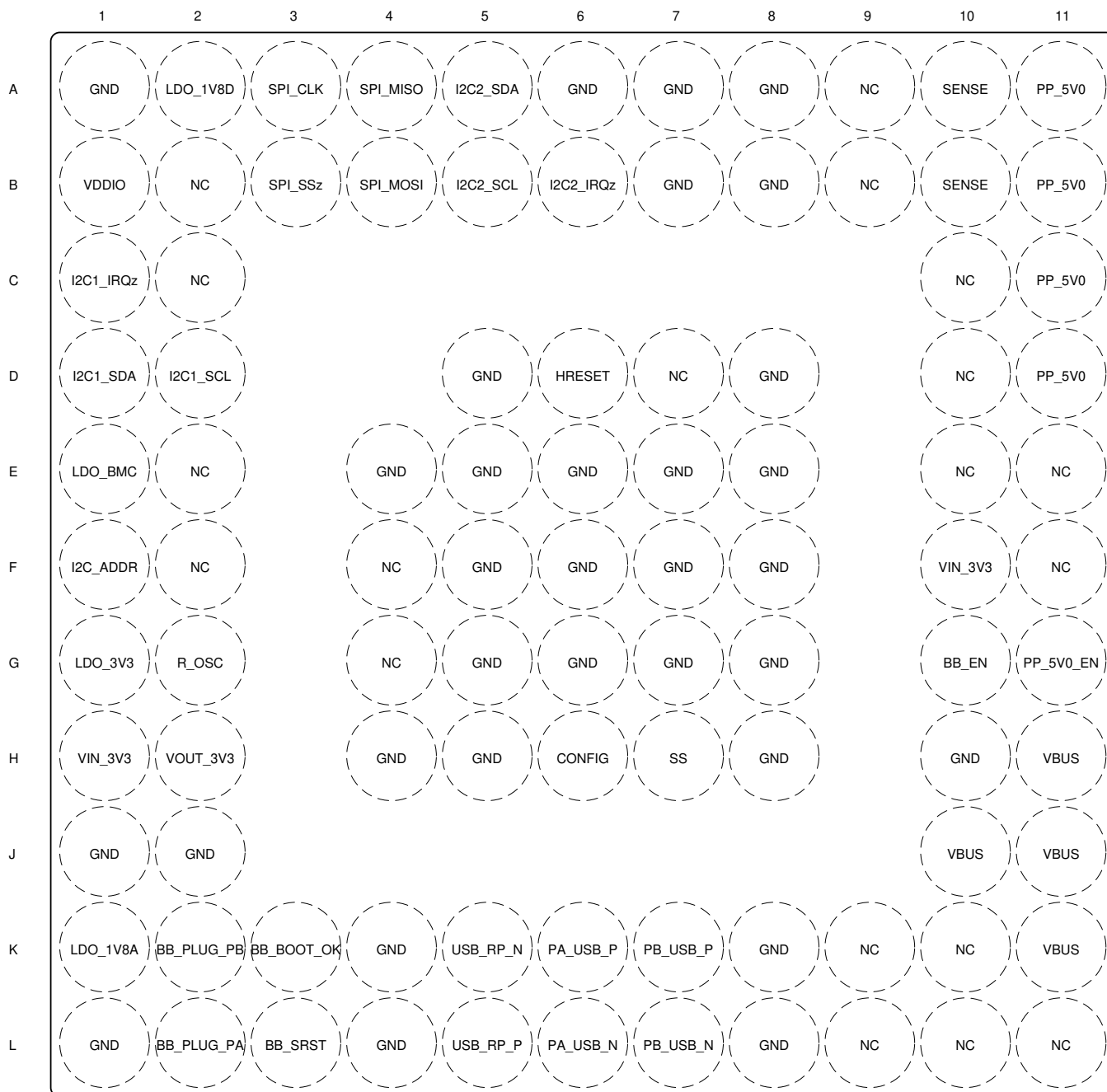
ZBH Package 96-Pin NFBGA Transparent Top View
