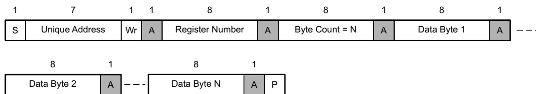
Figure 17. I 2 C Unique Address-Write Register Protocol
