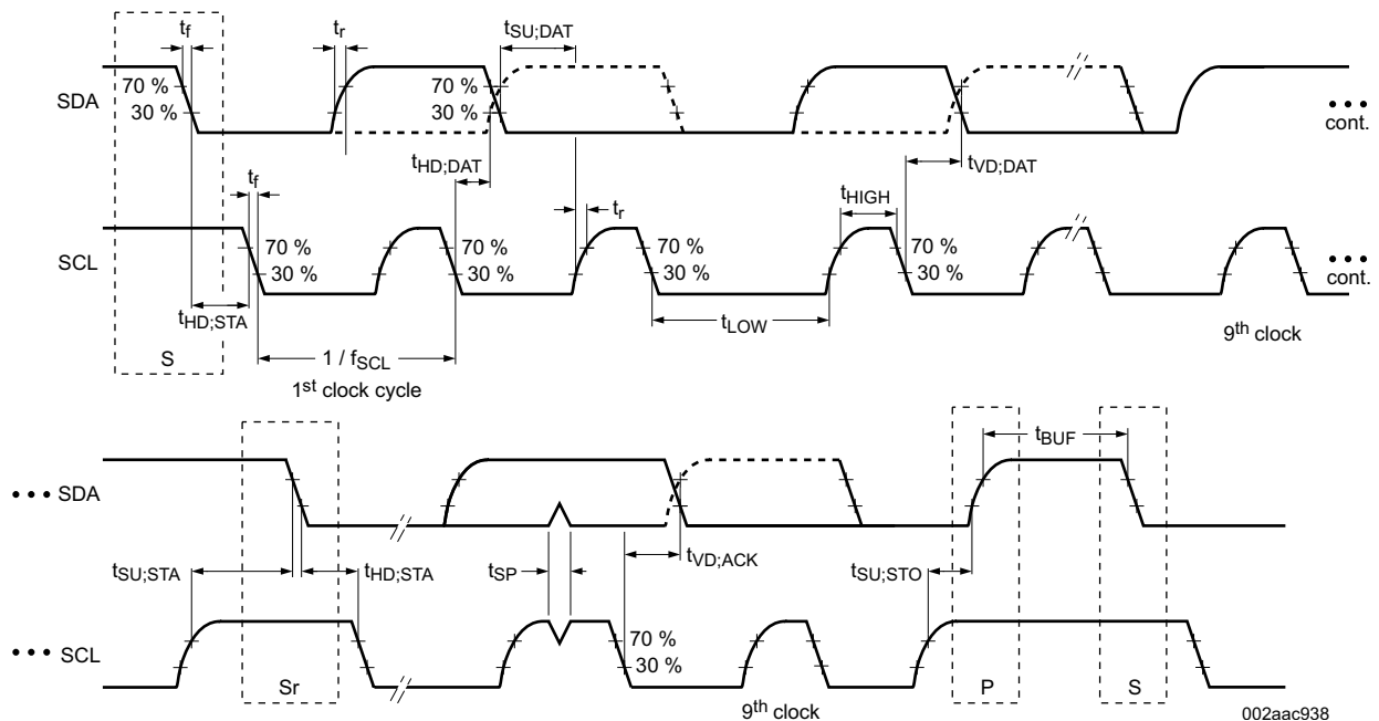
Figure 2. I²C Slave Interface Timing
