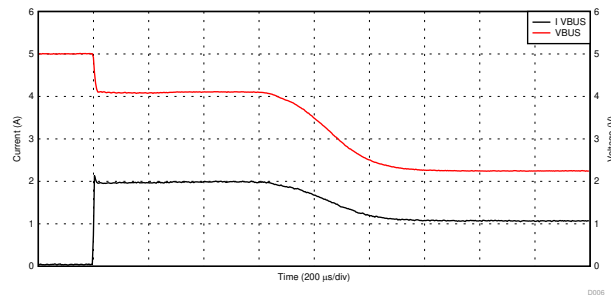
Figure 8. PP_5V0 Current Limit With a Soft Short (2 Ω)
