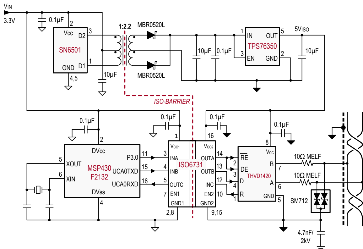
Figure 9-1. Isolated RS-485 Interface Circuit
