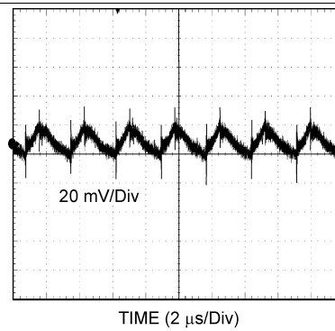
Figure 34. Output Ripple
