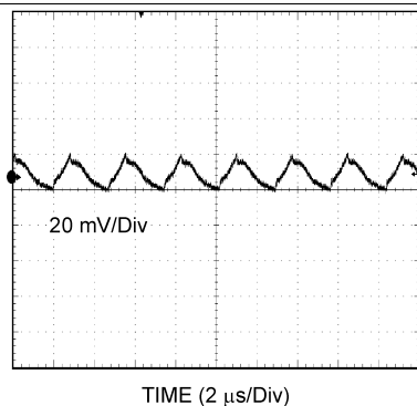
Figure 33. Output Ripple
