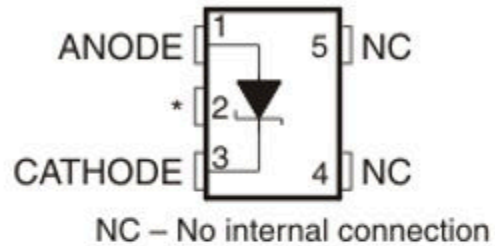
1.2 V...DCK (SC-70) PACKAGE (TOP VIEW)
