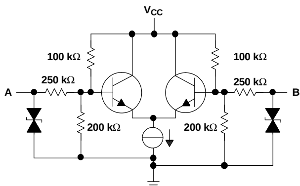
RECEIVER INPUT
