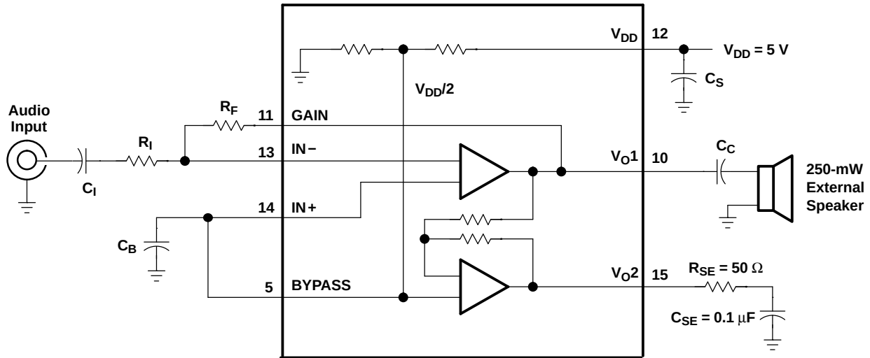
Figure 38. Singled-Ended Mode
