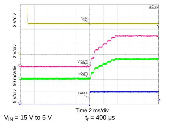
Figure 18. Recovery from OVP
