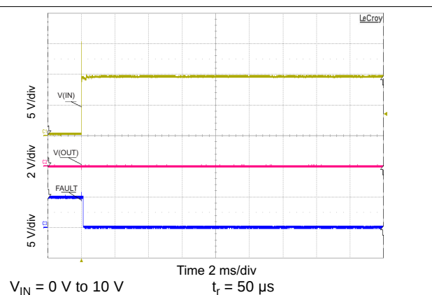
Figure 16. OVP at Power-On
