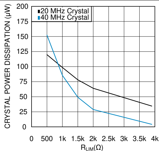
Figure 6-10. Crystal Power Dissipation vs. R_{\text{LIM}}
