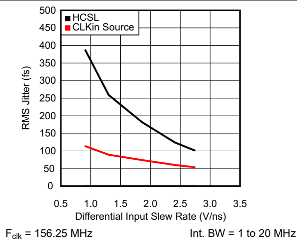
Figure 6-6. RMS Jitter vs. CLKIn Slew Rate at 156.25 MHz
