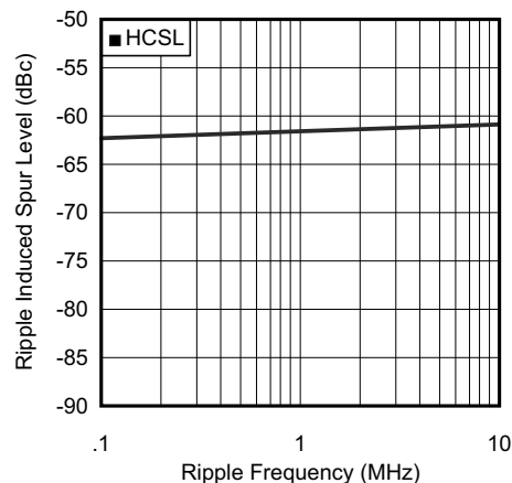
Figure 6-8. PSRR vs. Ripple Frequency at 312.5 MHz
