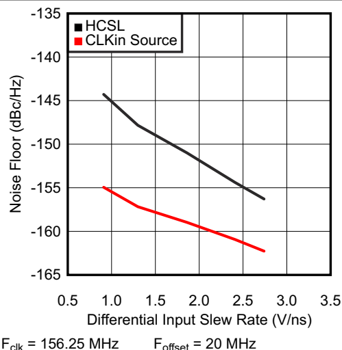
Figure 6-4. Noise Floor vs. CLKIn Slew Rate at 156.25 MHz
