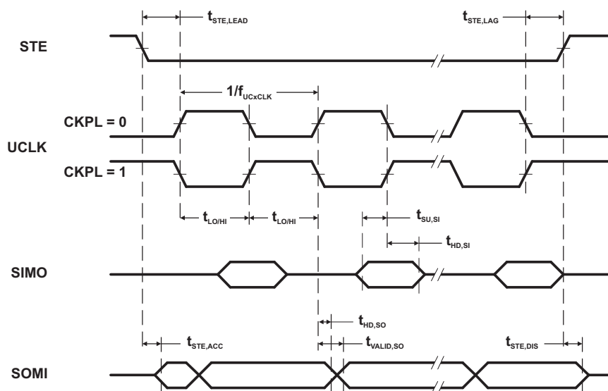
Figure 5-36. SPI Slave Mode, CKPH = 0
