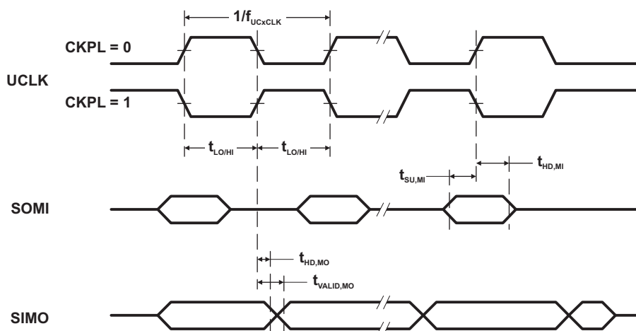
Figure 5-35. SPI Master Mode, CKPH = 1
