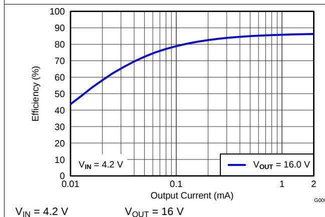
Figure 5-9. Boost Efficiency vs I_{OUT}
