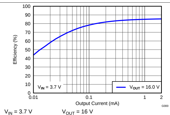
Figure 5-8. Boost Efficiency vs I_{OUT}
