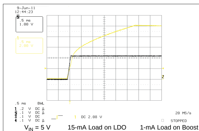
Figure 4-1. Startup
