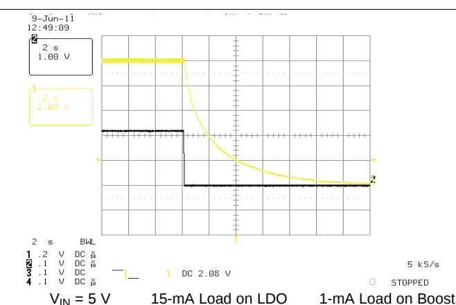
Figure 4-2. Shutdown
