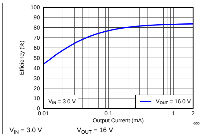
Figure 5-7. Boost Efficiency vs I_{OUT}
