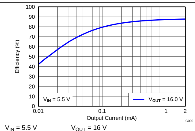
Figure 5-10. Boost Efficiency vs I_{OUT}
