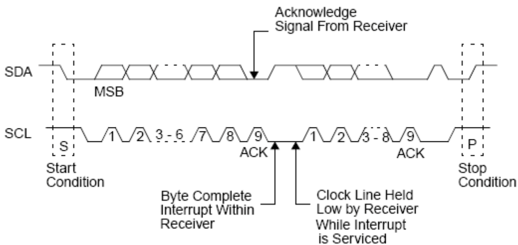
Figure 4. Acknowledge (ACK)
