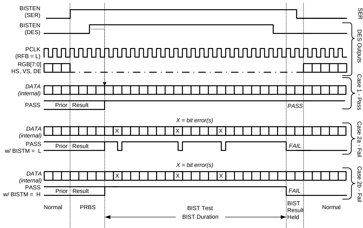
Figure 21. BIST Waveforms
