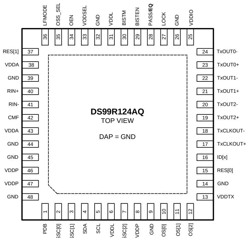
Figure 2. FPD-Link II to FPD-Link Convertor WQFN Package See package Number RHS0048A
