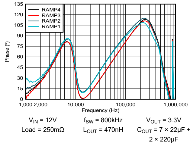
Figure 6-4. Phase versus Ramp Setting - VREF = 0.9V
