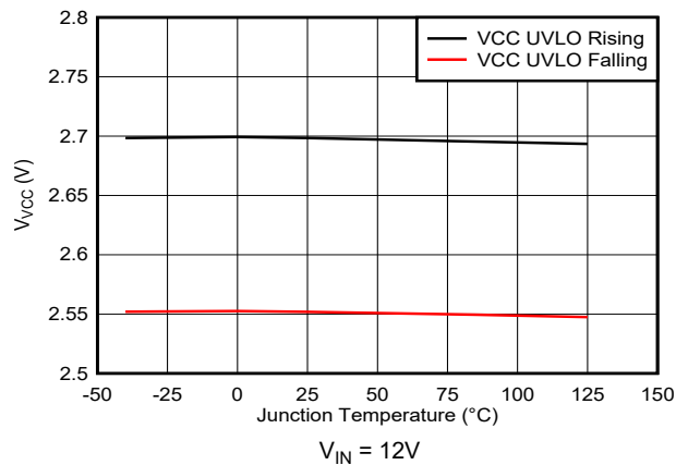
Figure 5-29. VCC Pin Undervoltage Lockout versus Junction Temperature
