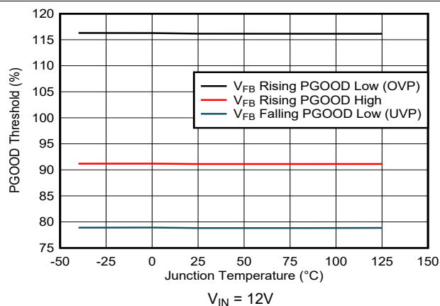
Figure 5-35. Power-Good Thresholds versus Junction Temperature ( V_{REF} = 0.5V )
