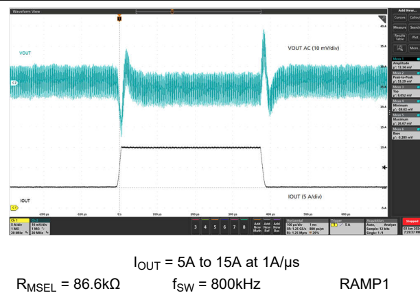
Figure 7-6. Load Transient
