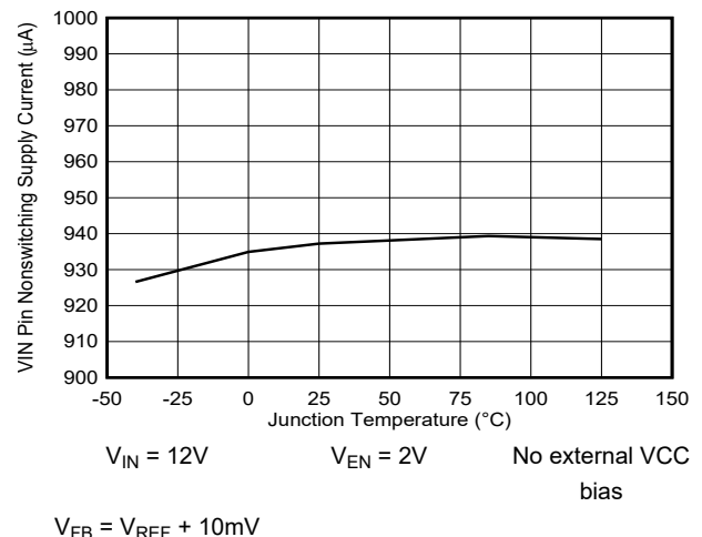
Figure 5-24. VIN Pin Nonswitching Quiescent Current versus Junction Temperature
