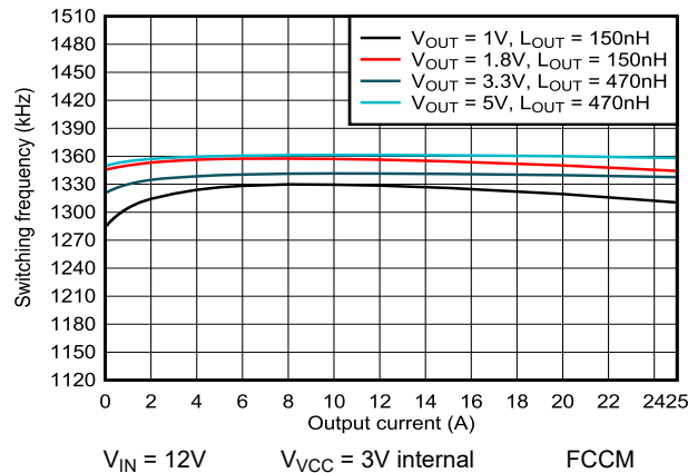
Figure 5-19. 1400kHz Switching Frequency versus Output Current
