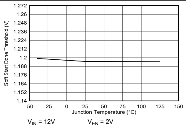
Figure 5-34. Soft-Start Done Voltage Threshold versus Junction Temperature ( V_{REF} = 0.9V )
