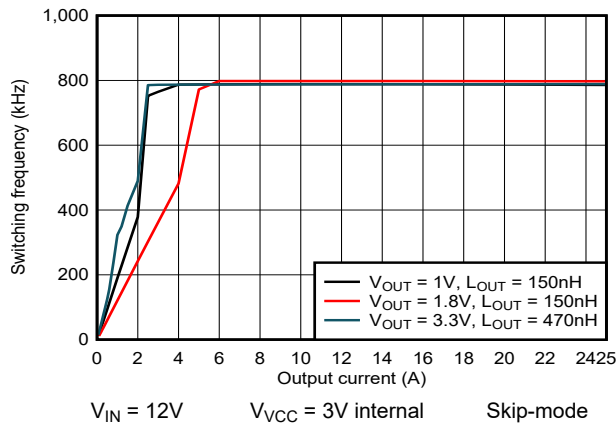
Figure 5-17. 800kHz Skip-mode Switching Frequency versus Output Current
