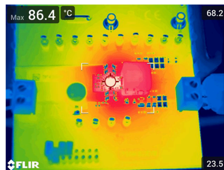
Figure 5-8. Thermal Image – 3.3V Output, TPS54KB20EVM, 6 Layers
