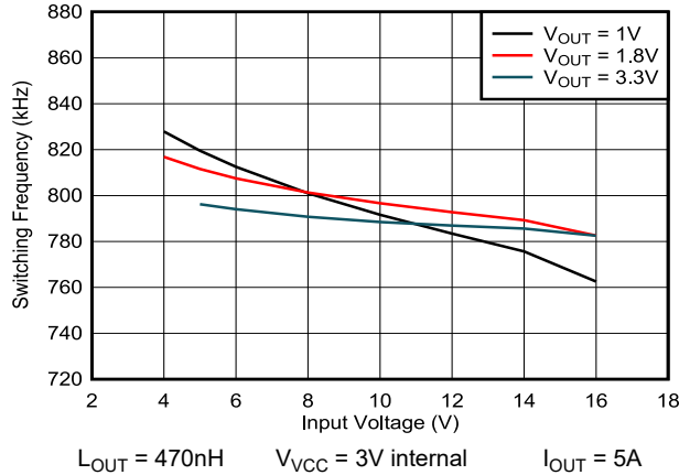
Figure 5-13. 800kHz Switching Frequency versus Input Voltage
