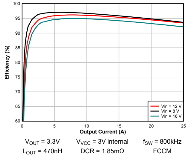
Figure 7-3. Efficiency – FCCM
