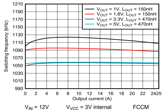
Figure 5-18. 1100kHz Switching Frequency versus Output Current
