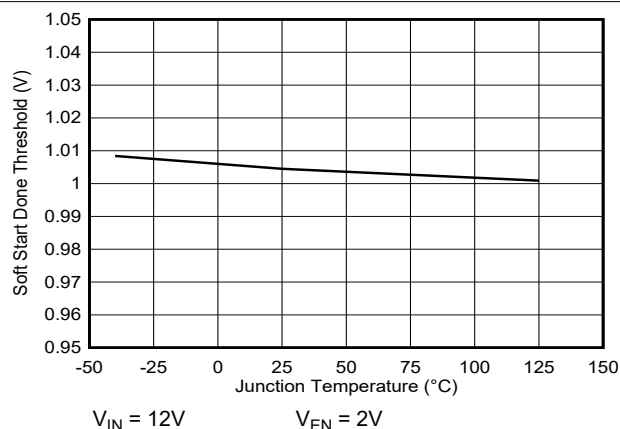
Figure 5-33. Soft-Start Done Voltage Threshold versus Junction Temperature ( V_{REF} = 0.5V )
