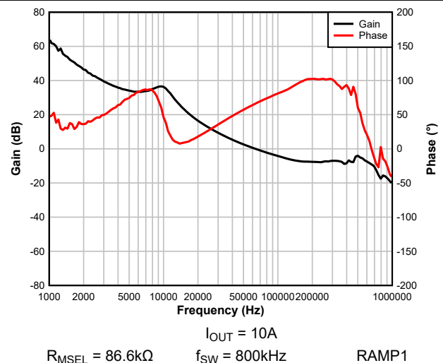
Figure 7-7. Bode Plot
