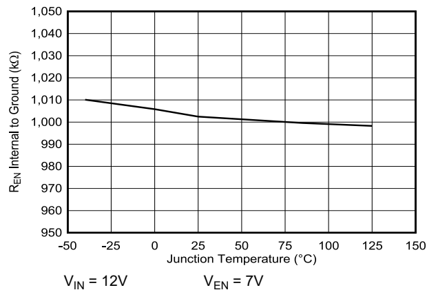
Figure 5-31. EN Pin Internal Resistance to Ground versus Junction Temperature
