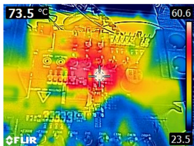
Figure 5-9. Thermal Image – 5V Output, 3 Inch x 3 Inch, 4 Layers
