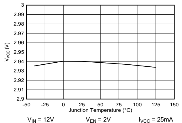
Figure 5-22. VCC Pin Output Voltage versus Junction Temperature
