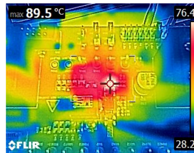
Figure 5-8. Thermal Image – 3.3V Output, TPS54KB20EVM, 6 Layers
