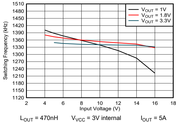
Figure 5-15. 1400kHz Switching Frequency versus Input Voltage
