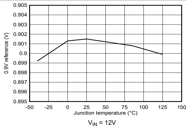
Figure 5-21. 0.9V Reference Voltage versus Junction Temperature
