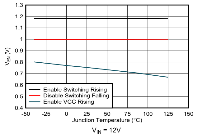
Figure 5-30. EN Pin Thresholds versus Junction Temperature
