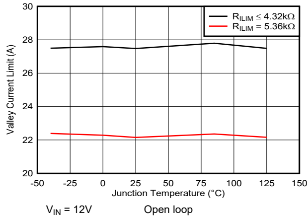
Figure 5-25. Valley Current Limit versus Junction Temperature (Low R_{ILIM} )
