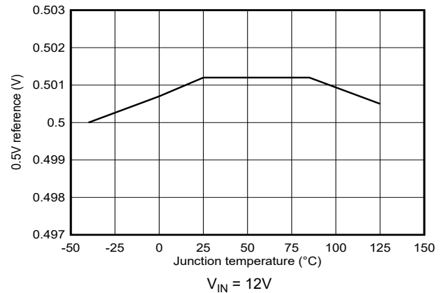
Figure 5-20. 0.5V Reference Voltage versus Junction Temperature
