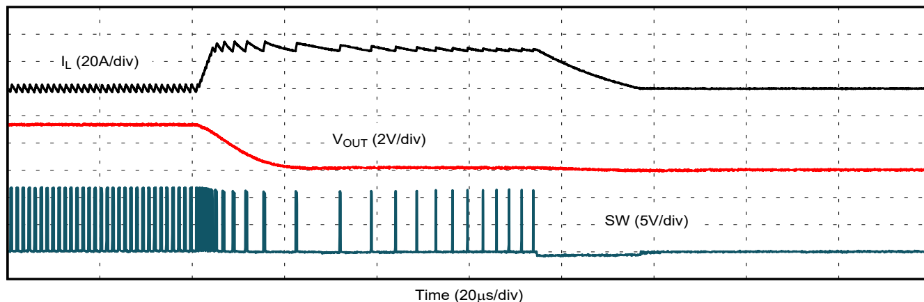
Figure 6-7. Overcurrent Protection
