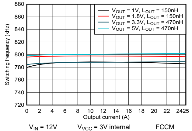
Figure 5-16. 800kHz FCCM Switching Frequency versus Output Current
