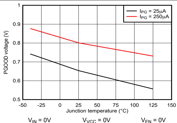
Figure 5-37. Power-Good Clamp Voltage versus Junction Temperature
