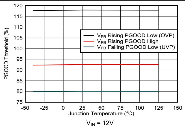
Figure 5-36. Power-Good Thresholds versus Junction Temperature ( V_{REF} = 0.9V )
