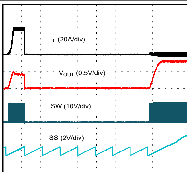
Figure 6-2. Exiting Hiccup
