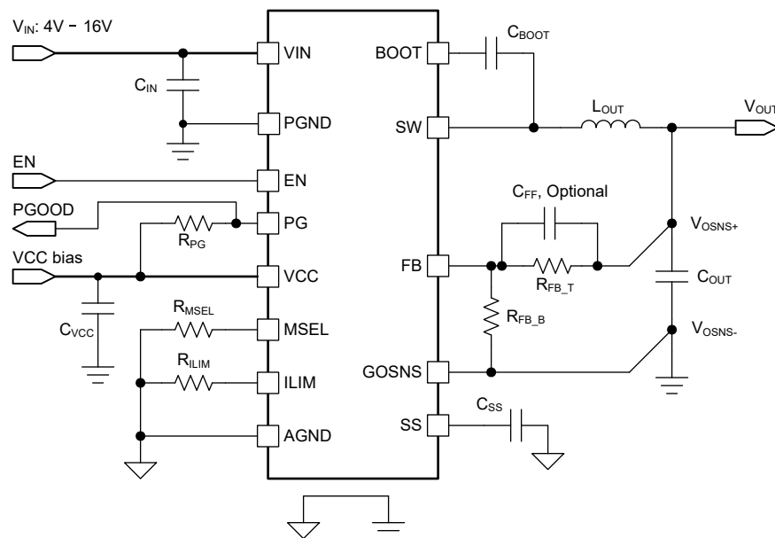
Figure 6-10. Split-Rail Configuration With External VCC Bias
