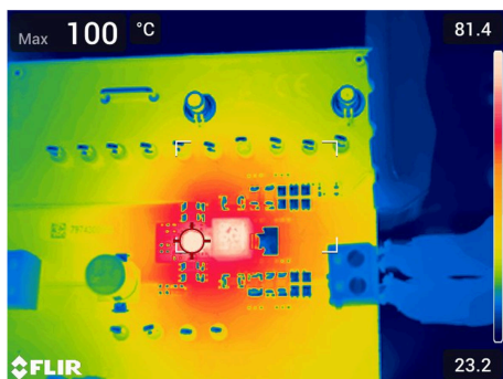
Figure 5-7. Thermal Image – 5V Output, TPS54KB20EVM, 6 Layers
