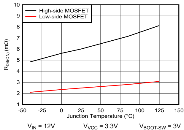
Figure 5-27. MOSFET R_{DS(ON)} versus Junction Temperature
