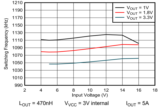
Figure 5-14. 1100kHz Switching Frequency versus Input Voltage
