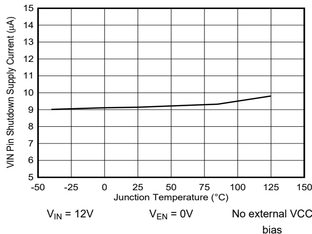
Figure 5-23. VIN Pin Shutdown Quiescent Current versus Junction Temperature
