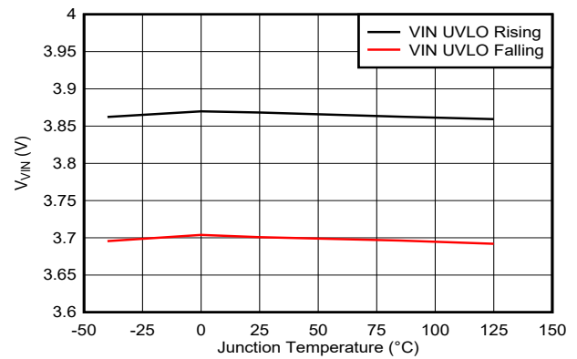
Figure 5-28. VIN Pin Undervoltage Lockout versus Junction Temperature
