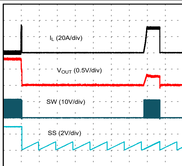
Figure 6-1. Entering Hiccup
