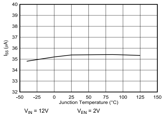
Figure 5-32. SS Pin Output Current versus Junction Temperature
