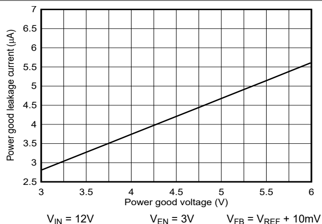
Figure 5-38. Power-Good Leakage Current versus Power-Good Voltage
