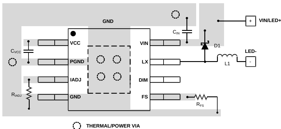
Figure 25. Layout Recommendation
