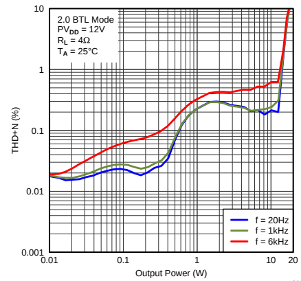
Figure 18. THD+N vs Output Power
