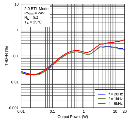
Figure 22. THD+N vs Output Power
