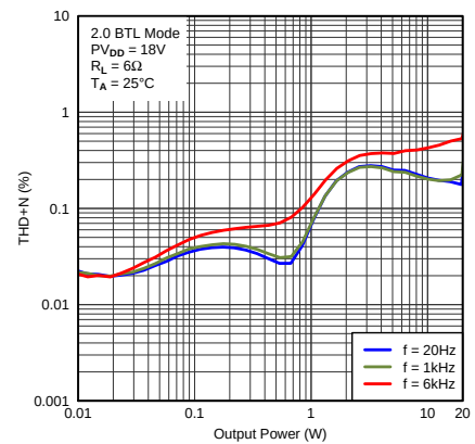
Figure 20. THD+N vs Output Power
