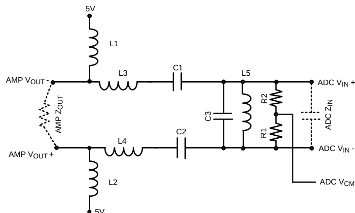
Figure 51. Sample Filter
