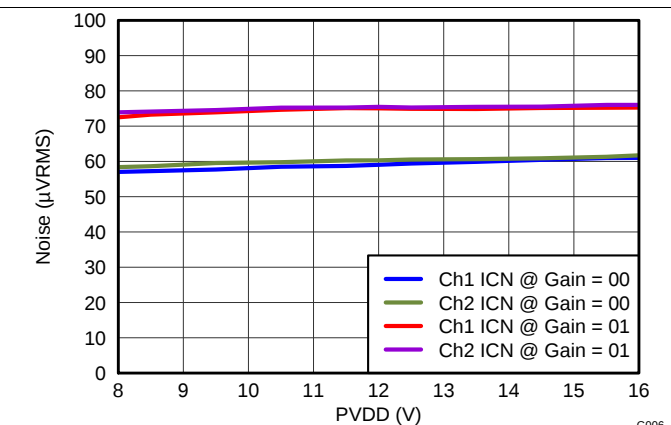
Figure 17. Idle Channel Noise vs PVDD
