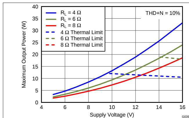
Figure 14. Output Power vs PVDD
