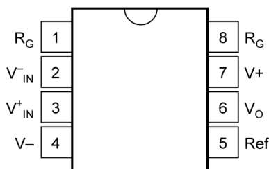
Figure 4-2. P Package, 8-Pin PDIP (Top View)
