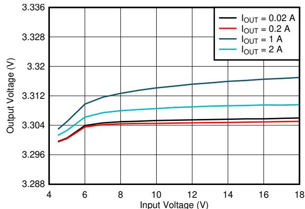
Figure 8-4. Line Regulation
