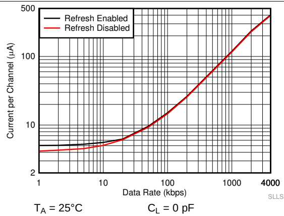
Figure 9. ISO7041 Supply Current vs Data Rate at 5 V (With No Load)
