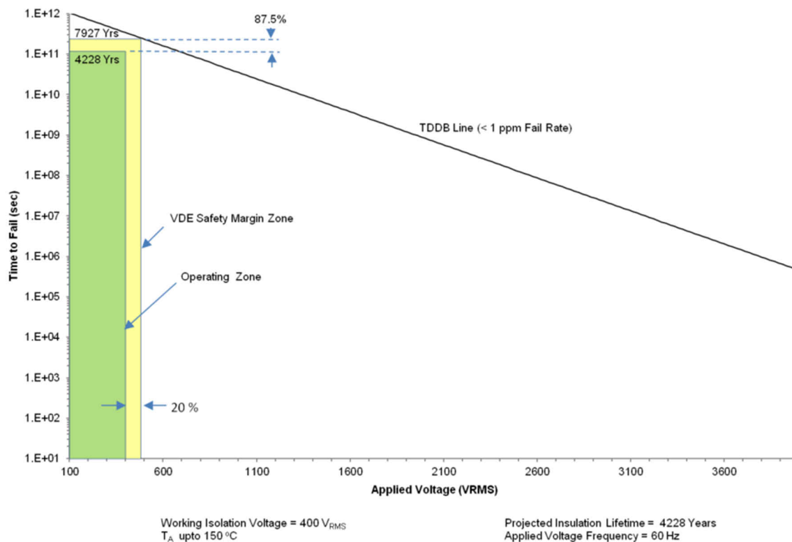
Figure 9-2. Insulation Lifetime Projection Data
