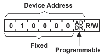
Figure 7-7. TCAL6416 Address
