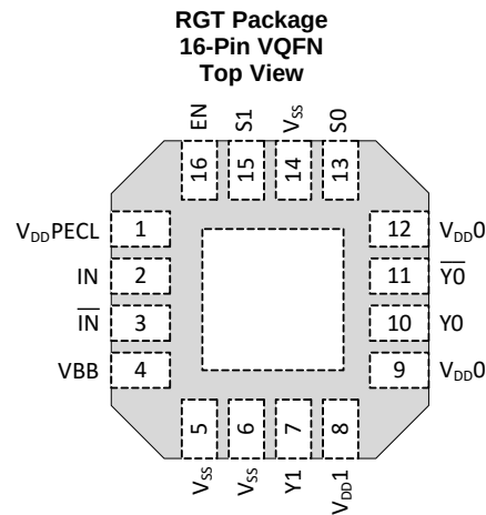
Pin Functions
