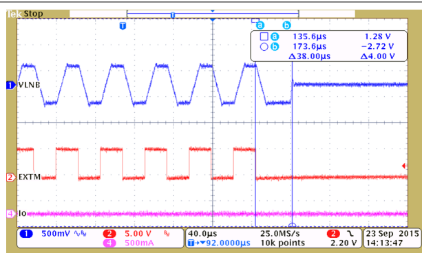
Figure 8-13. No load, 22 kHz Tone Delay from EXTIN 22 kHz Input Turns Low To Output Tone Off
