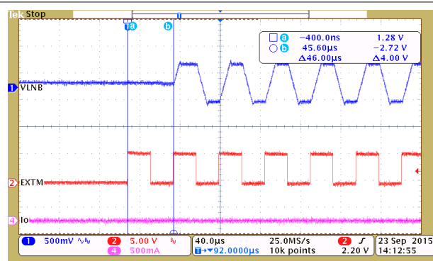
Figure 8-12. No load, 22 kHz Tone Delay from EXTIN 22 kHz Input Turns High To Output Tone On
