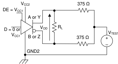
Figure 8-1. Driver Voltages
