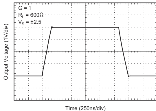
Figure 6-19. Large-Signal Step Response
