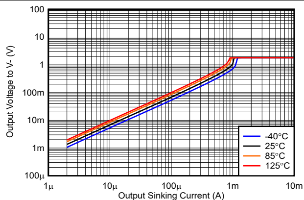
Figure 5-14. Output Voltage vs. Output Sinking Current, 1.8V
