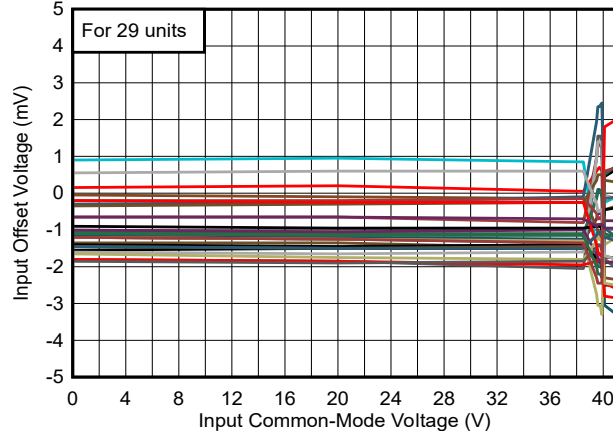
Figure 5-7. Offset vs. Common-Mode, 40V
