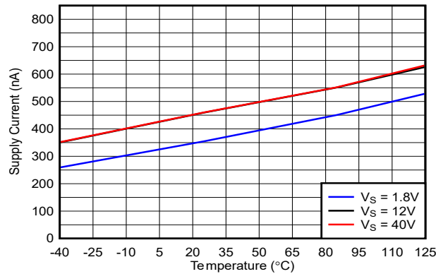
Figure 5-23. Supply Current vs. Temperature (Output Low), Push-Pull
