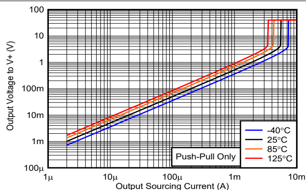
Figure 5-17. Output Voltage vs. Output Sourcing Current, 40V
