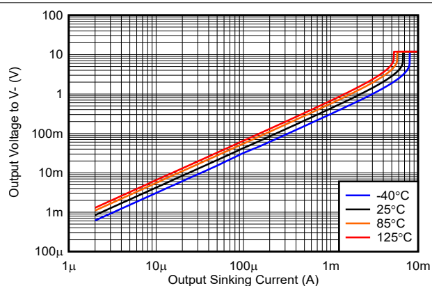
Figure 5-16. Output Voltage vs. Output Sinking Current, 12V
