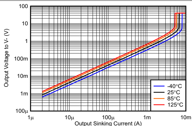
Figure 5-18. Output Voltage vs. Output Sinking Current, 40V
