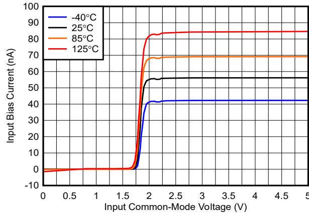
Figure 5-9. Bias Current vs. Common-Mode, 1.8V
