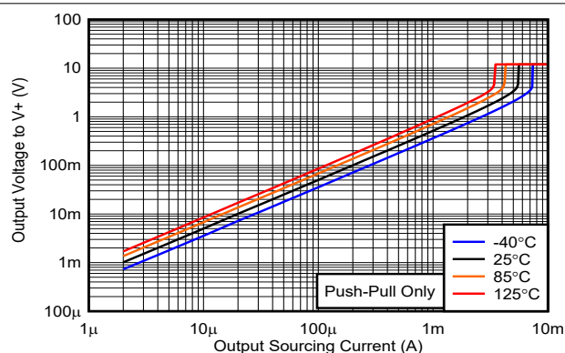
Figure 5-15. Output Voltage vs. Output Sourcing Current, 12V
