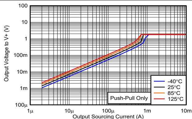
Figure 5-13. Output Voltage vs. Output Sourcing Current, 1.8V
