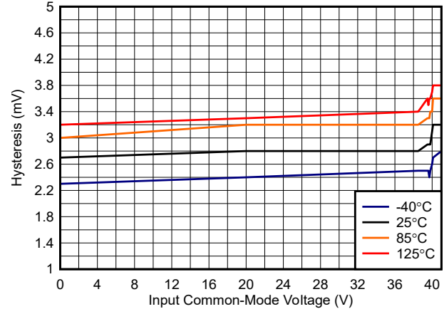
Figure 5-8. Hysteresis vs. Common-Mode, 40V
