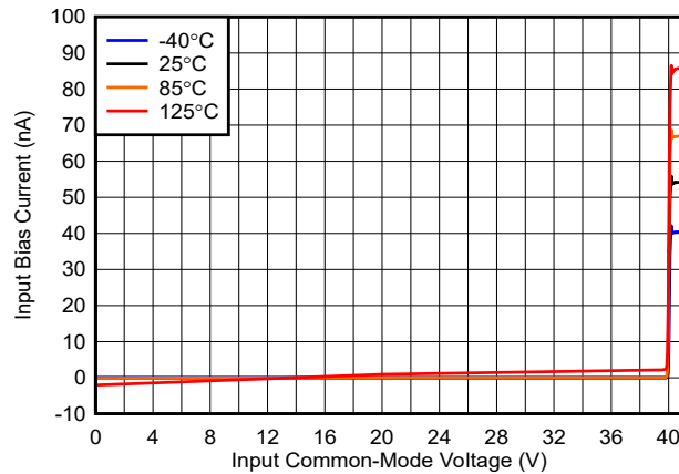
Figure 5-11. Bias Current vs. Common-Mode, 40V
