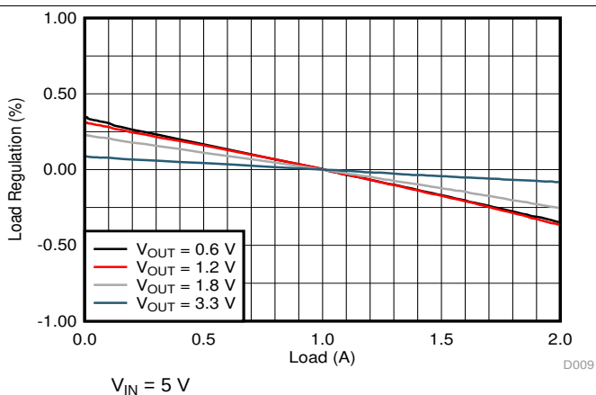
Figure 14. Load Regulation
