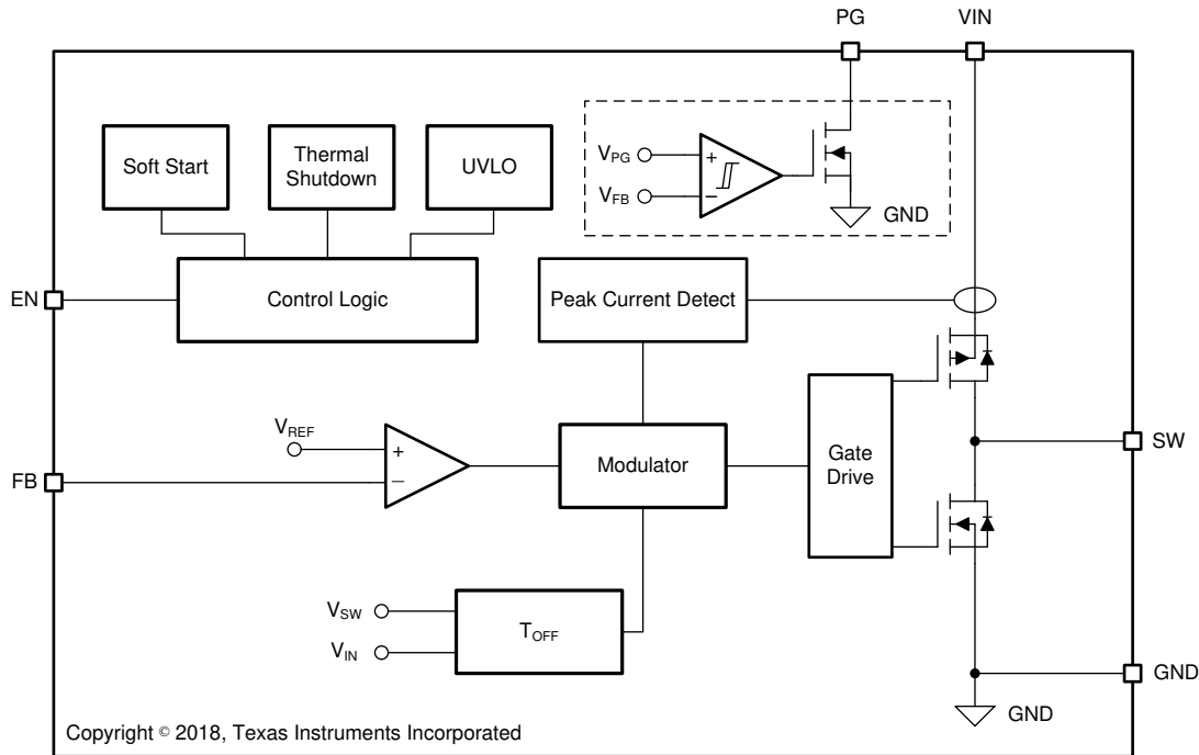
Figure 5. TLV62569A Functional Block Diagram
