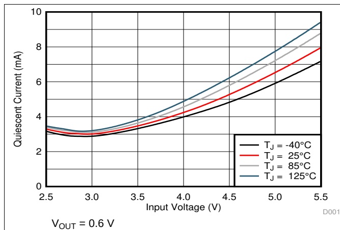
Figure 7. Quiescent Current
