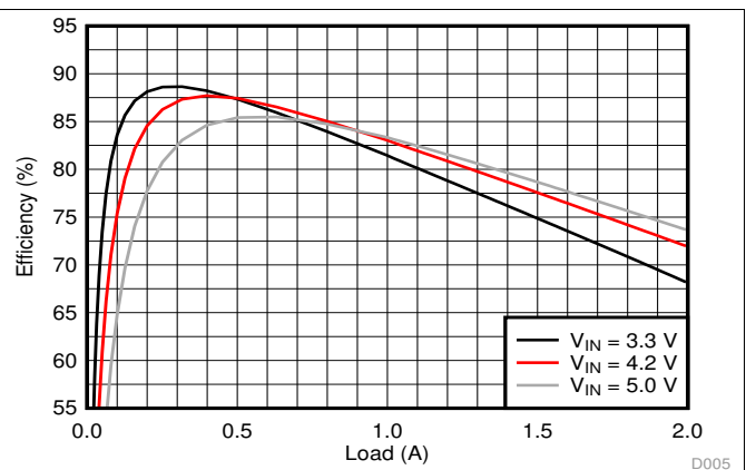
Figure 8. 0.6-V Output Efficiency
