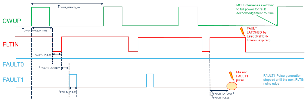
Figure 16. FAULTx lines integrity check in level mode (example with FAULT0 cyclic BIST disabled)
