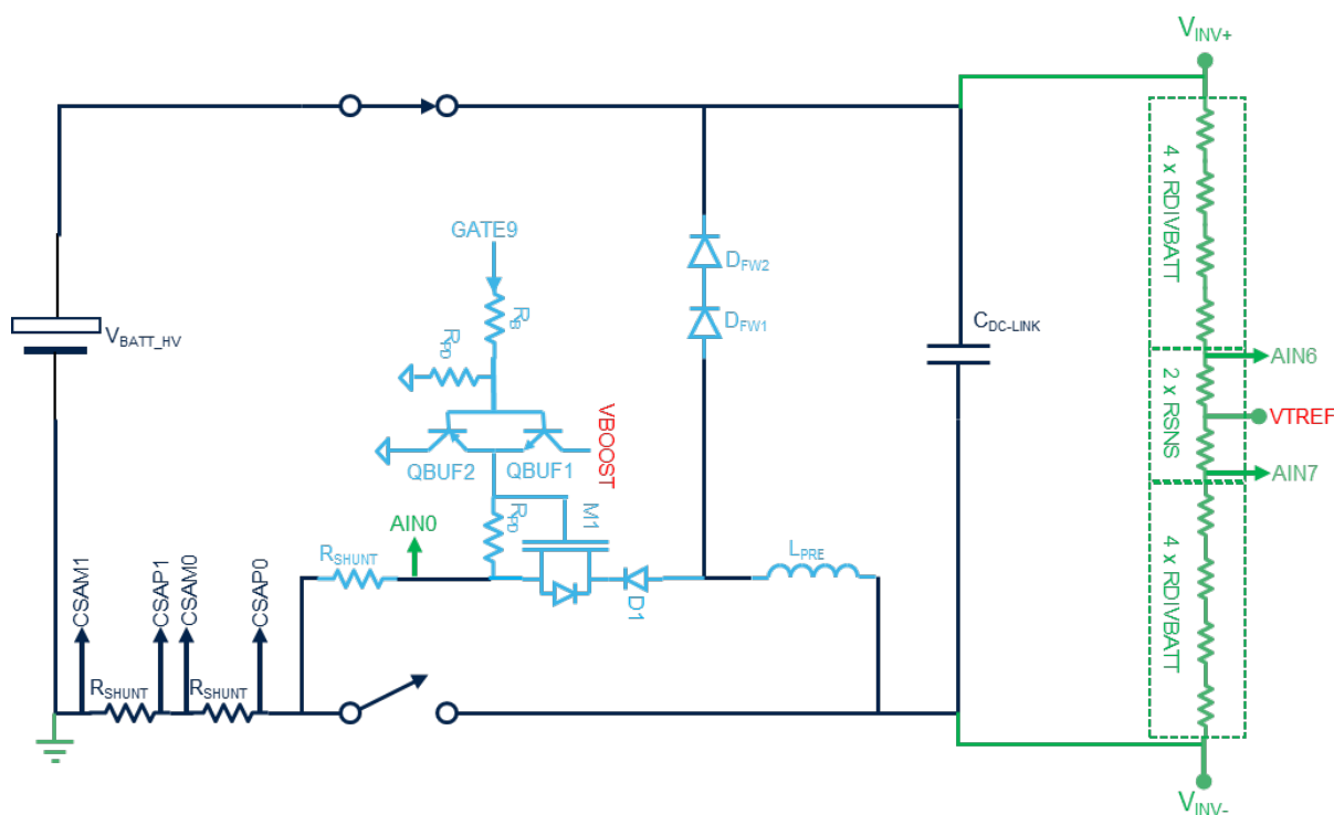
Figure 28. DC-Link precharge controller reference design
