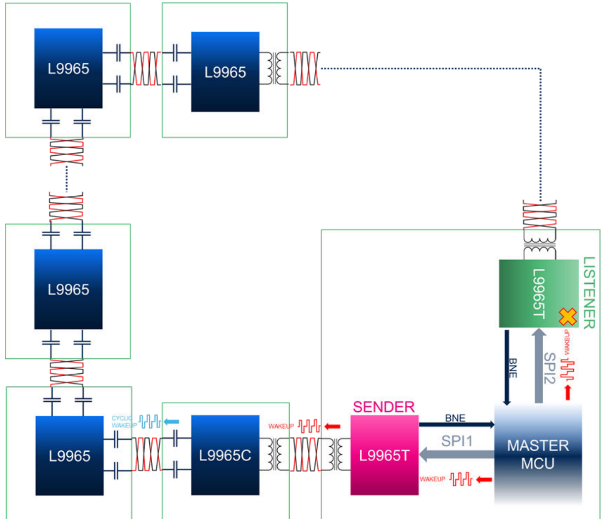
Figure 23. Wakeup by MCU
