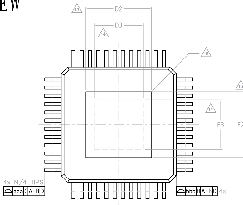
Figure 31. TQFP48L (7x7x1 mm exposed pad down) package outline - top and bottom
