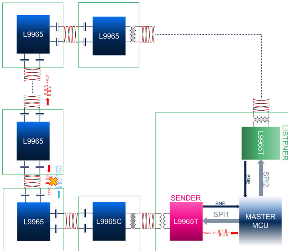
Figure 24. Wakeup by Fault
