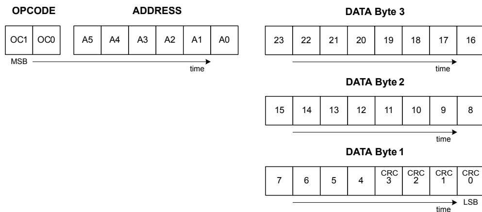
Figure 42. SDI frame
