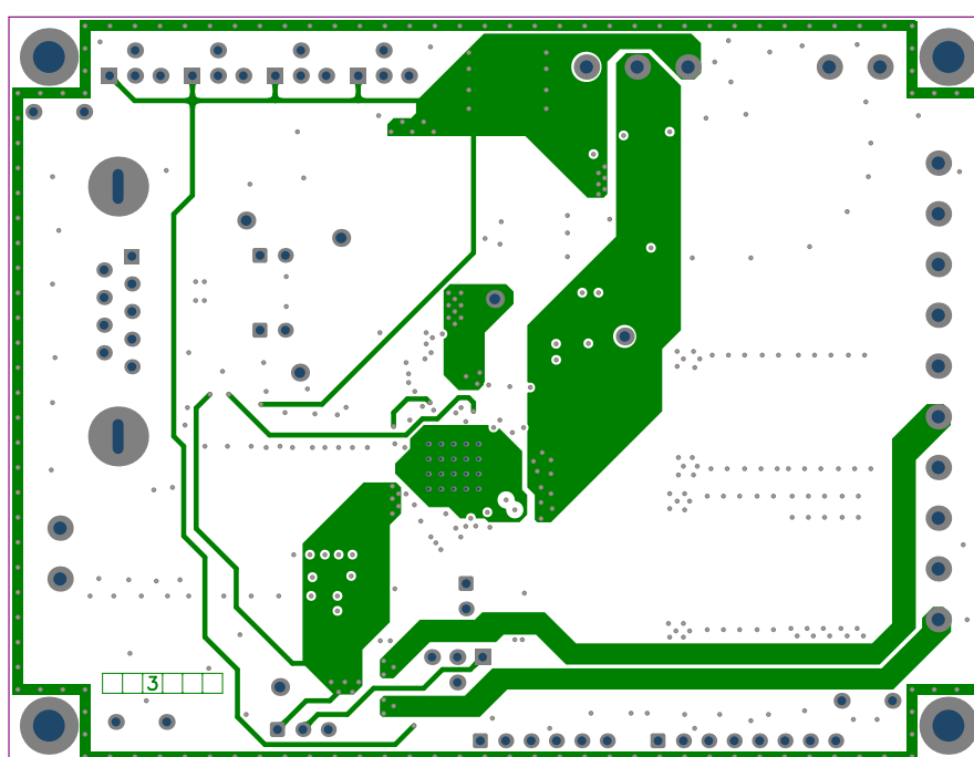
Figure 76. SPSB100G 6-Layer Demo Board – Layer 3
