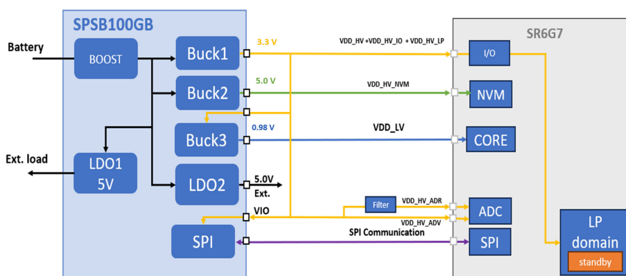
Figure 8. SPSB100GB direct supply of the microcontroller core
