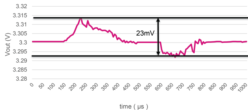
Figure 56. Buck1&2 @ 2.4 MHz
