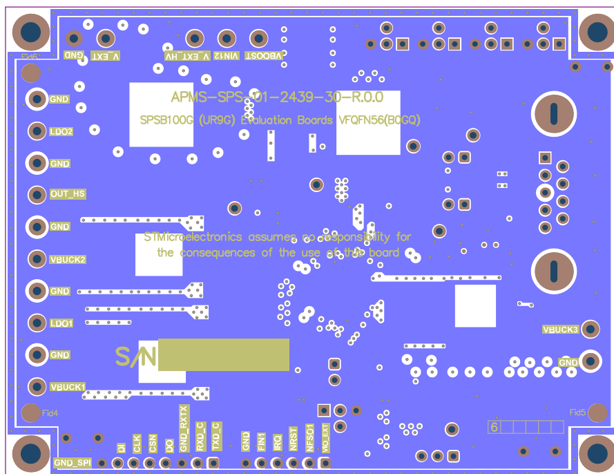
Figure 79. SPSB100G 6-Layer Demo Board – Bottom Layer
