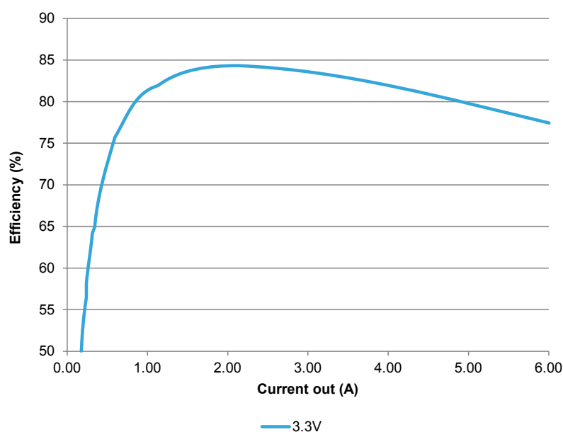
Figure 61. Buck3 efficiency VIN 3.30 V
