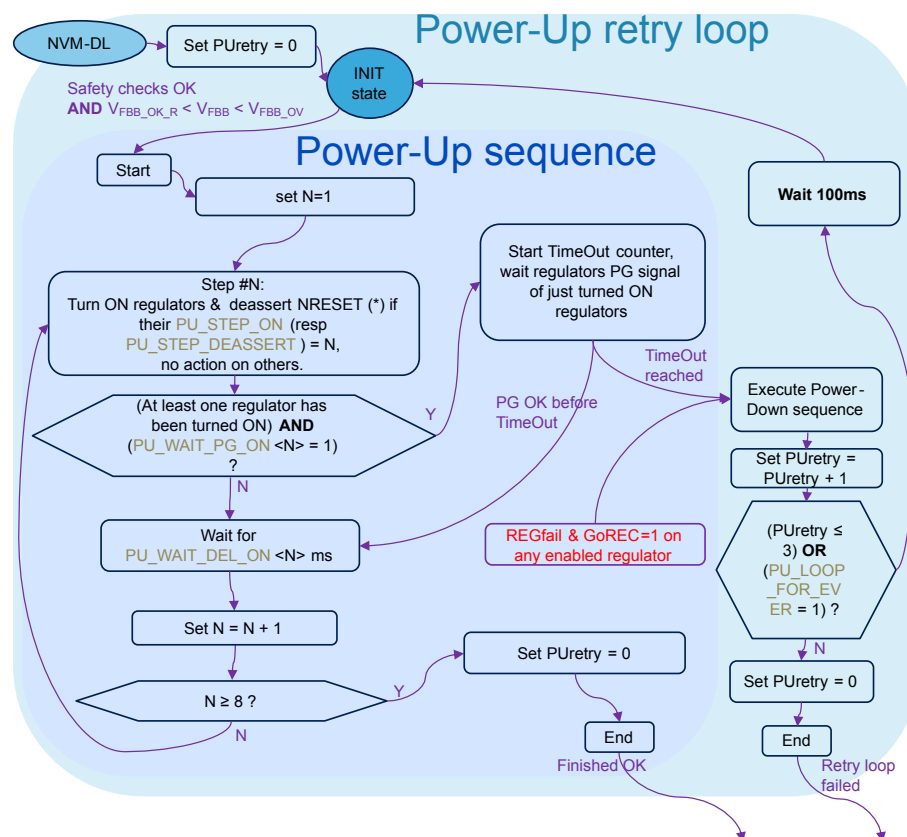
Figure 27. Power-up sequence
