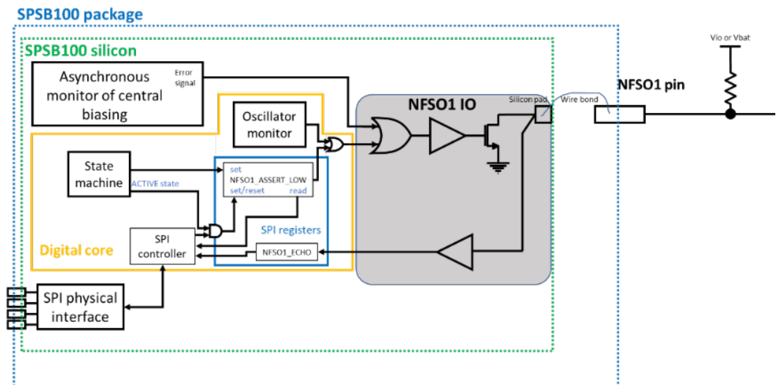
Figure 31. NFSO1 implementation details
