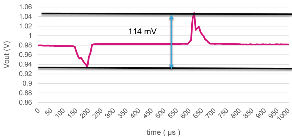
Figure 63. Buck3
