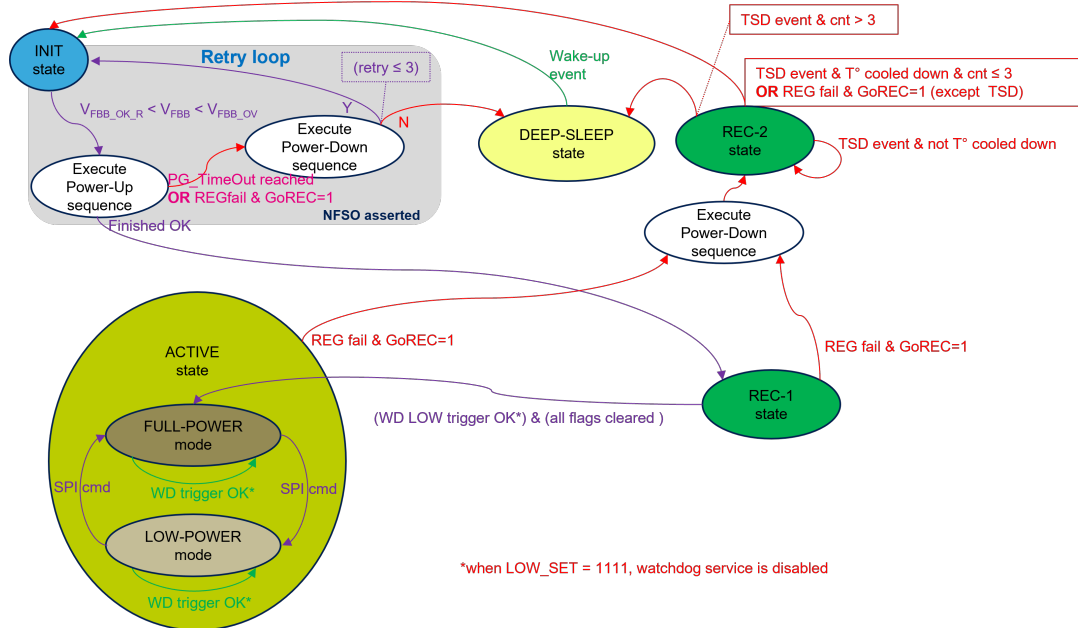
Figure 22. Regulator fault reaction with REGFAIL_GO_REC = 1
