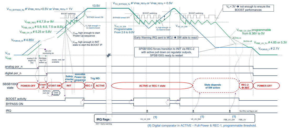
Figure 12. Battery drop behavior
