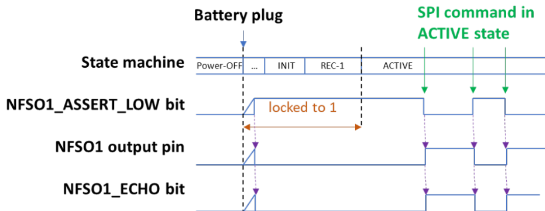
Figure 32. NFSO1 output pin behavior at battery plug
