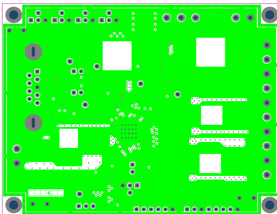
Figure 78. SPSB100G 6-Layer Demo Board – Layer 5
