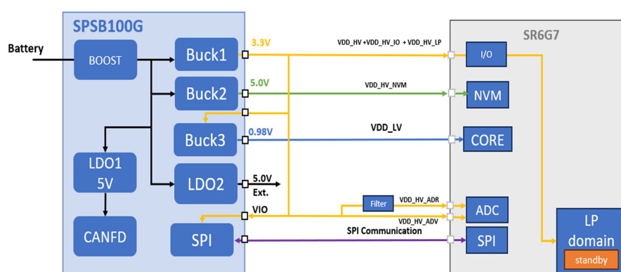
Figure 7. SPSB100G direct supply of the microcontroller core
