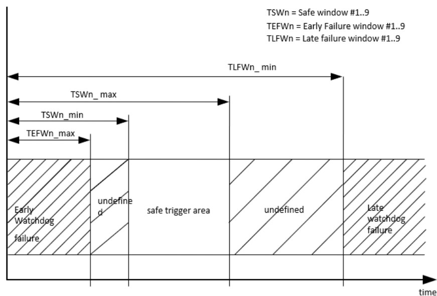
Figure 66. Watchdog early, late and safe windows
