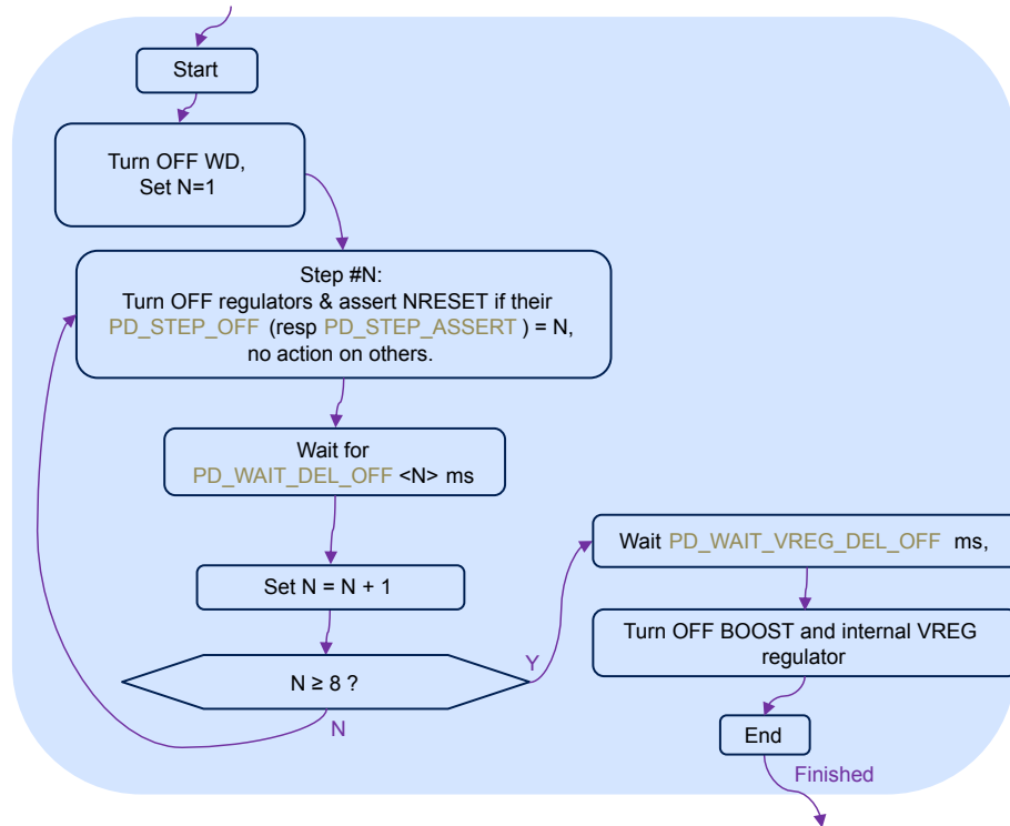
Figure 28. Power-down sequence
