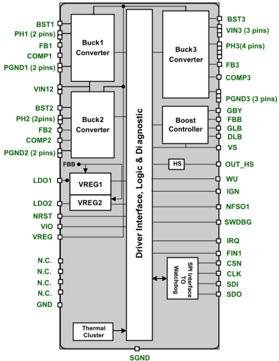
Figure 2. SPSB100GB block diagram
