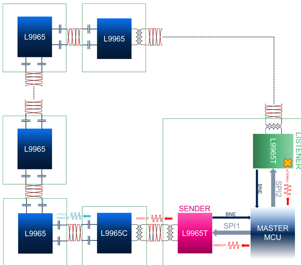
Figure 15. Wakeup by MCU
