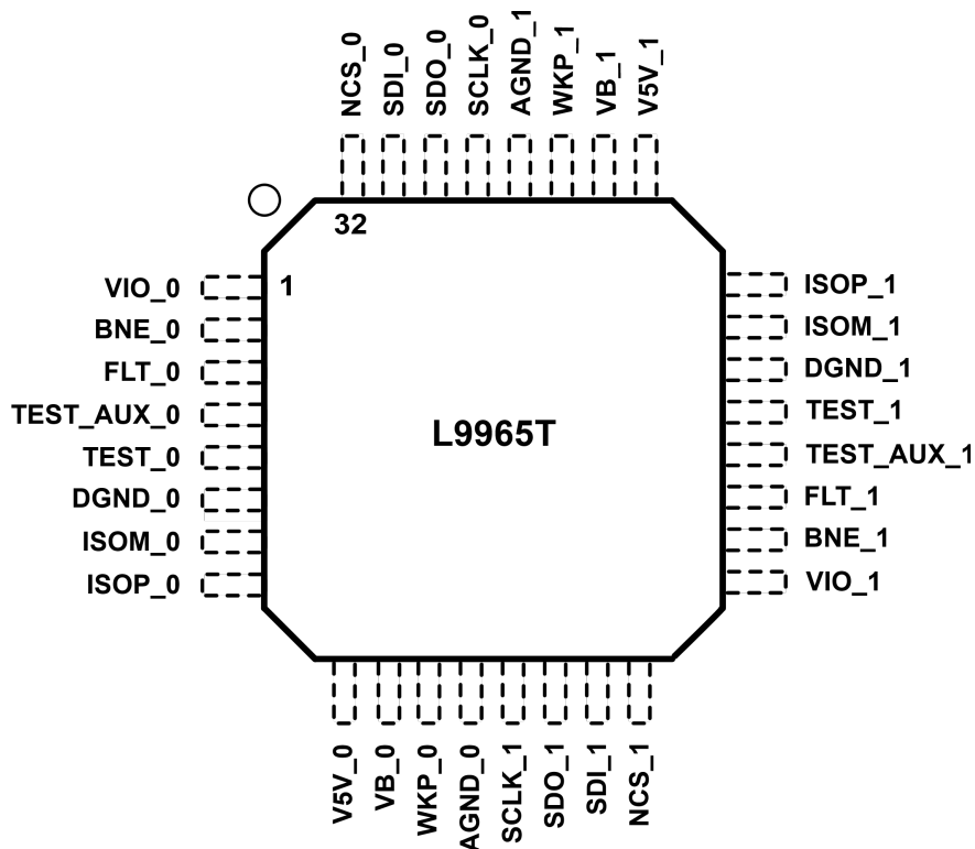
Figure 3. Pinout L9965T (top view)
