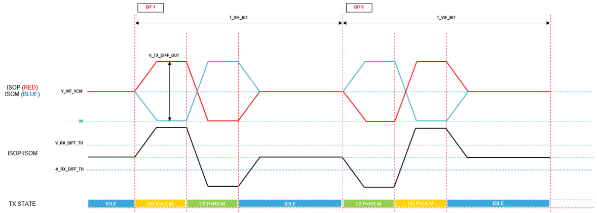
Figure 10. VIF waveform
