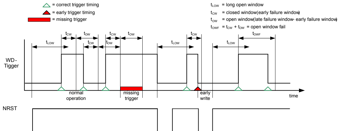
Figure 45. Window watchdog operation
