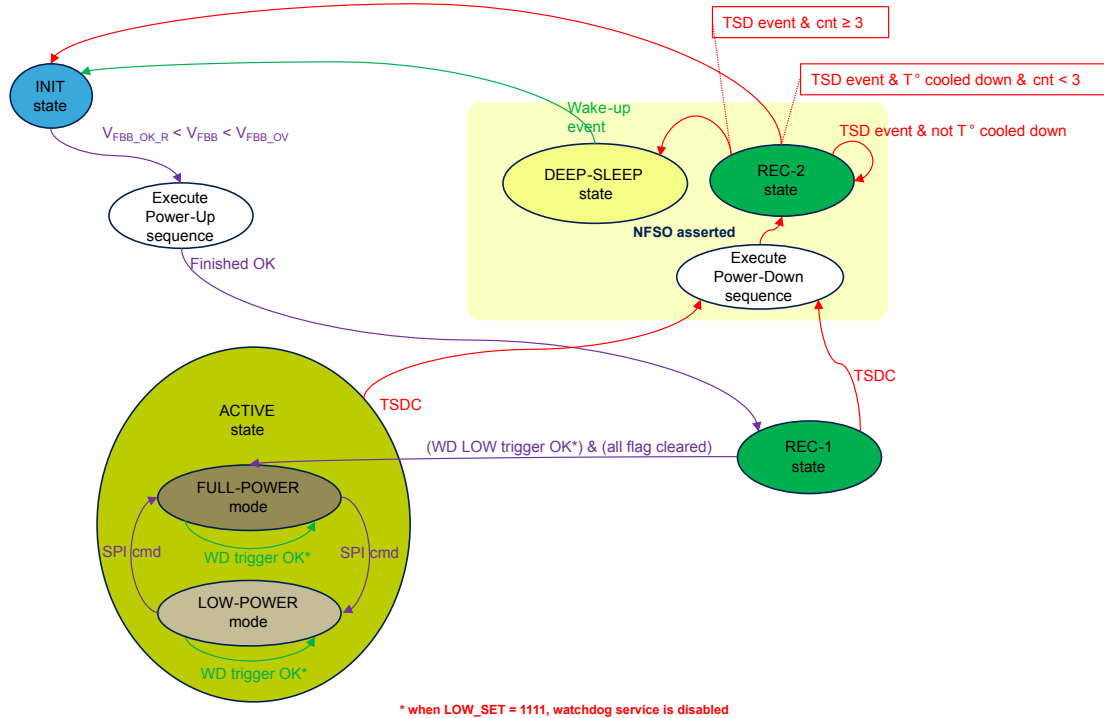
Figure 21. State machine details on TSDC fault
