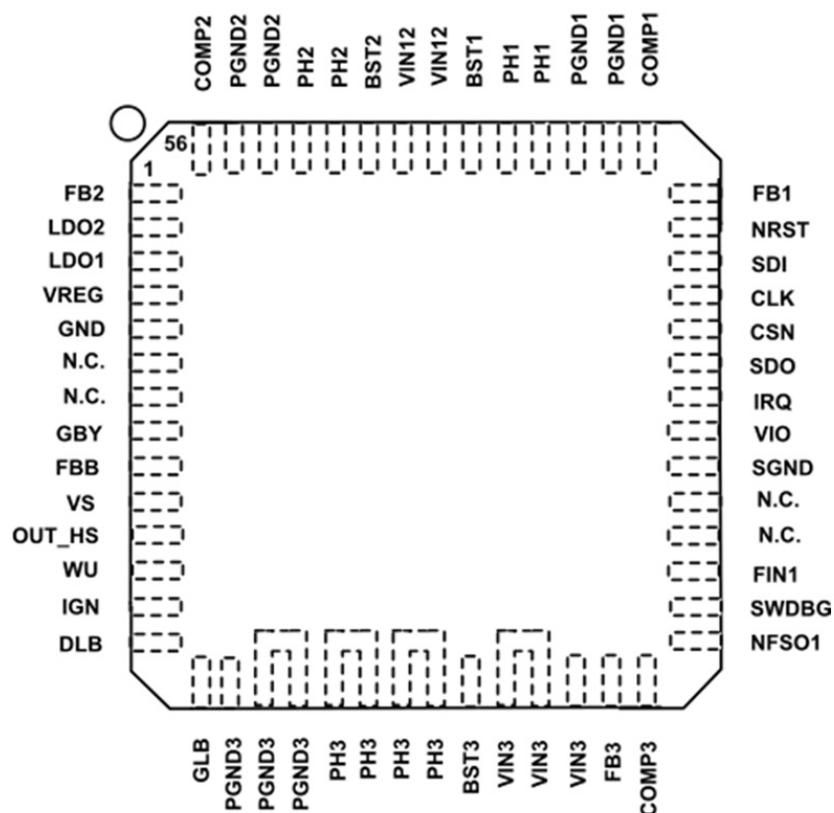
Figure 4. SPSB100GS pin connection (top view)
