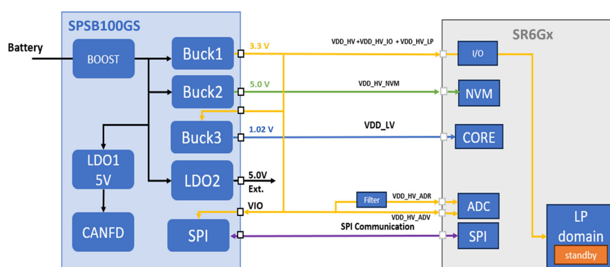
Figure 7. SPSB100GS direct supply of the microcontroller core
