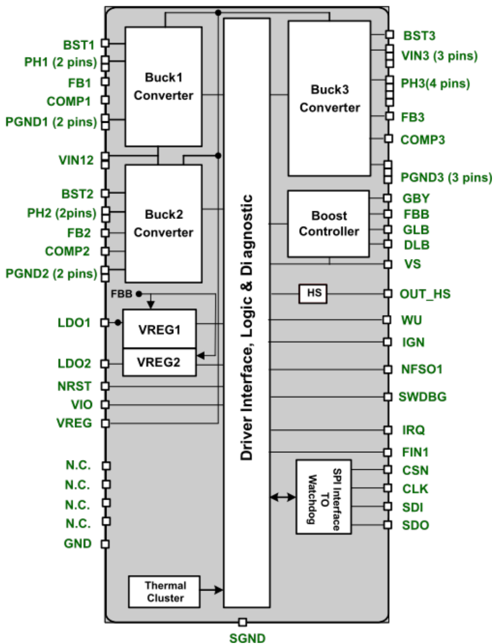
Figure 2. SPSB100GBS block diagram
