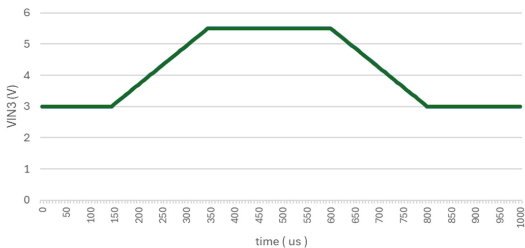
Figure 64. Buck3
