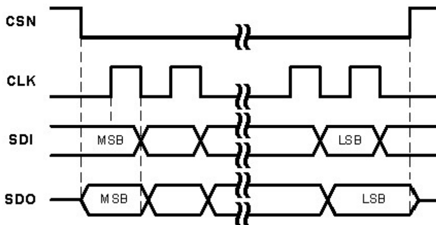
Figure 41. SPI signal description
