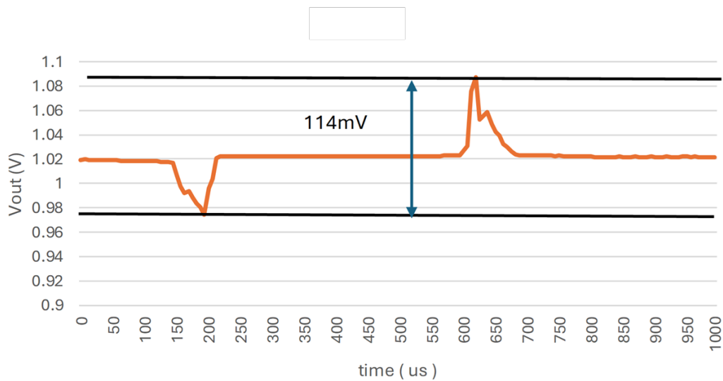
Figure 62. Buck3
