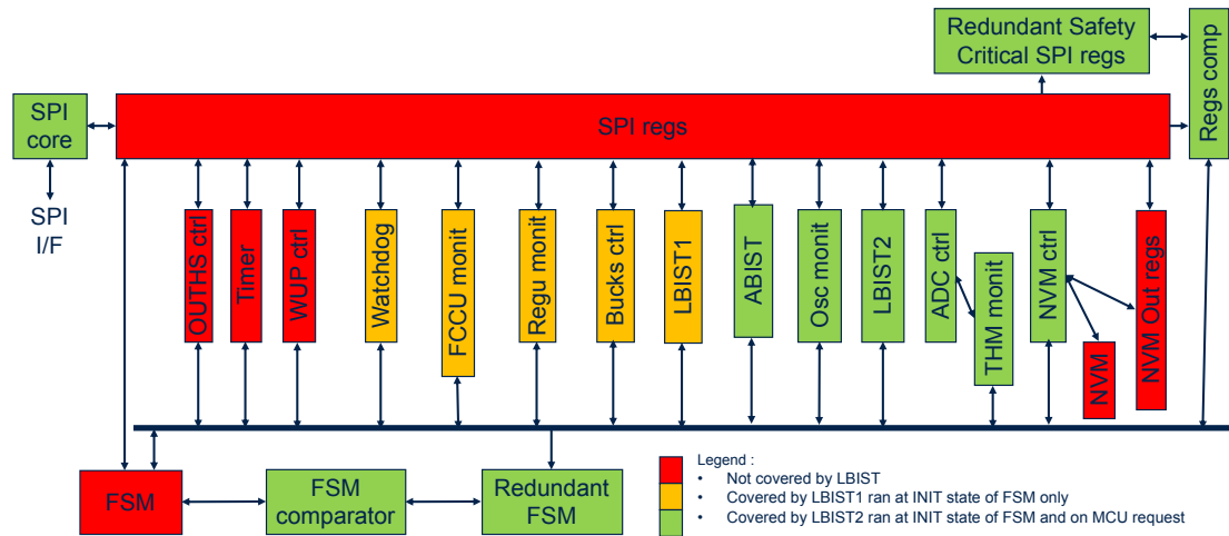
Figure 39. Logic BIST
