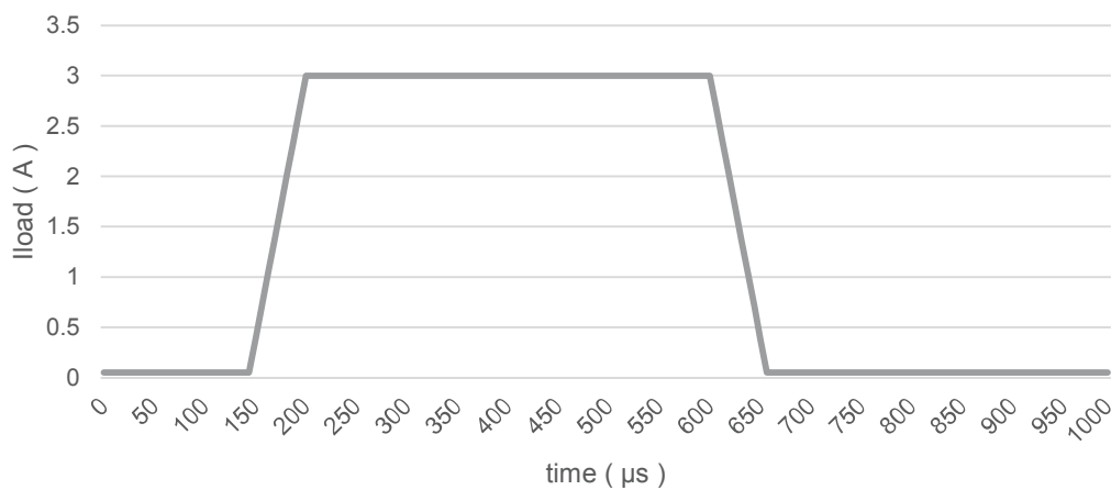
Figure 62. Buck3
