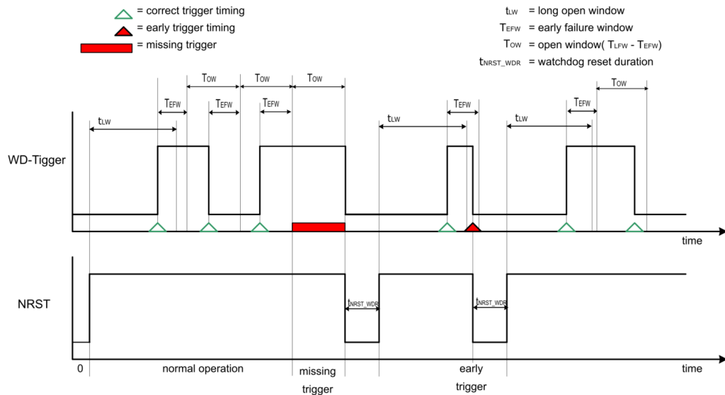
Figure 66. Watchdog timing
