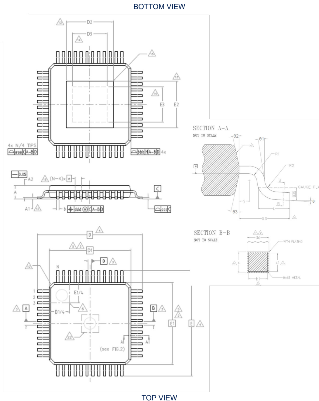
Figure 24. TQFP 7x7 48L EXPOSED PAD DOWN
