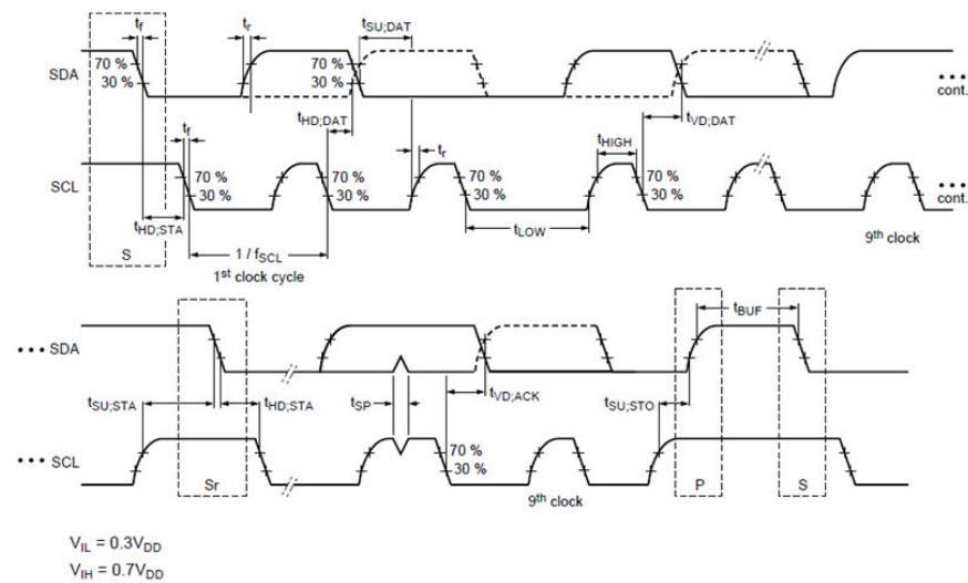
Figure 14. Timing on the I 2 C bus
