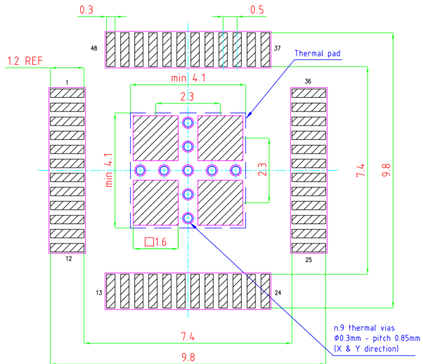
Figure 25. Proposed PCB landpattern
