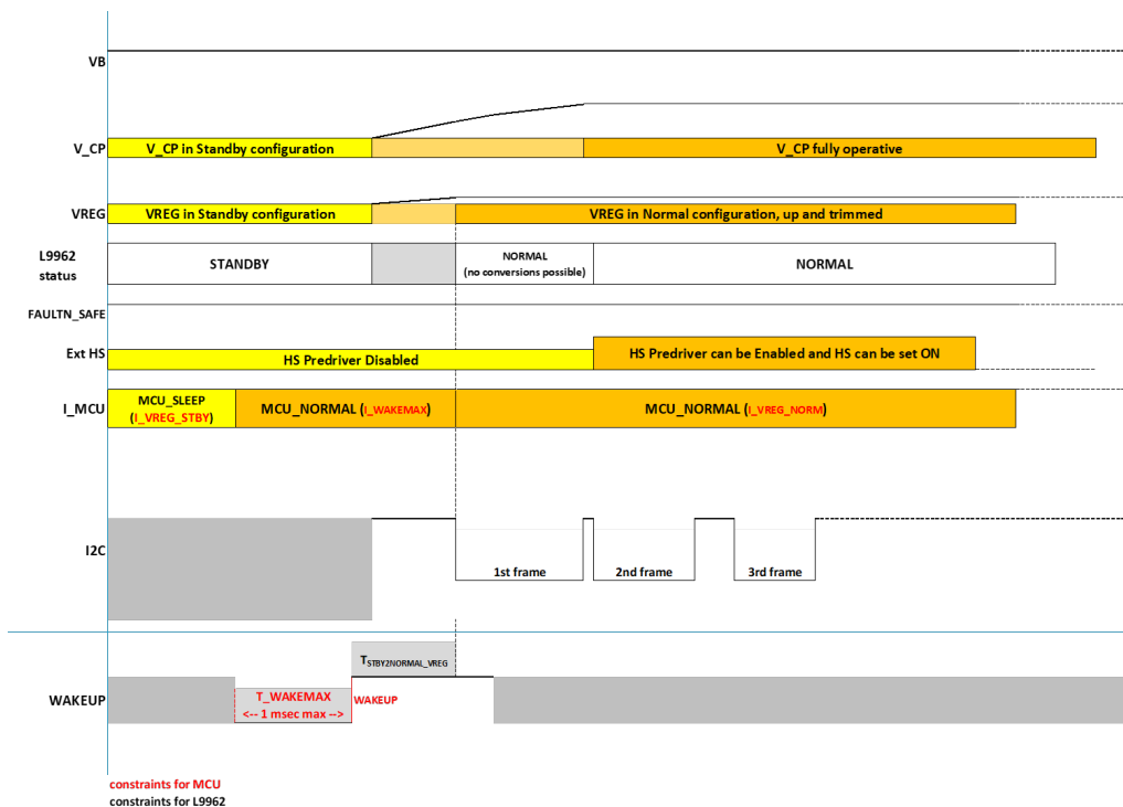
Figure 4. Timing diagram: transition from STANDBY to NORMAL upon WAKEUP detection
